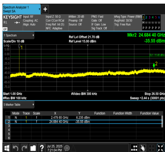
3DH5-Ant10-2480-1000~26500-PASS
