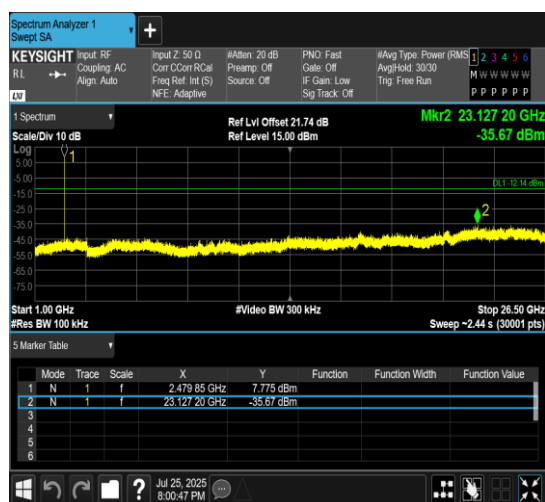
3DH5-Ant7-2480-1000~26500-PASS
