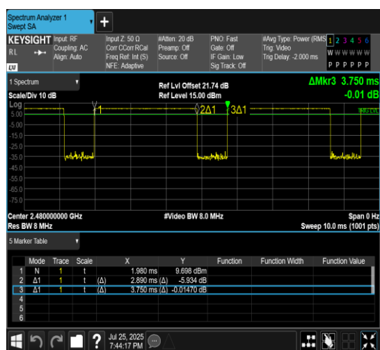
NTNV-DH5-Ant7-2480
