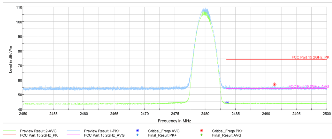
Fig.63. Frequency Band Edges: 8DPSK, Channel 78, 2.45 GHz - 2.50GHz
