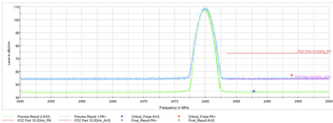
Fig.61. Frequency Band Edges: \pi/4 DQPSK, Channel 78, Hopping Off, 2.45 GHz - 2.50GHz
