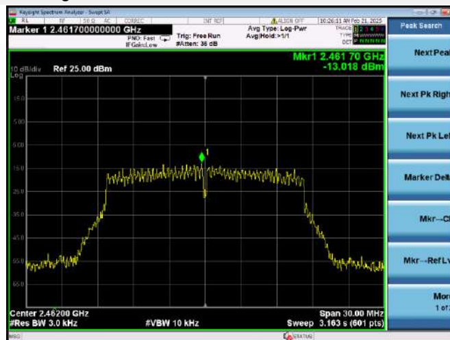
802.11g CHANNEL 11
