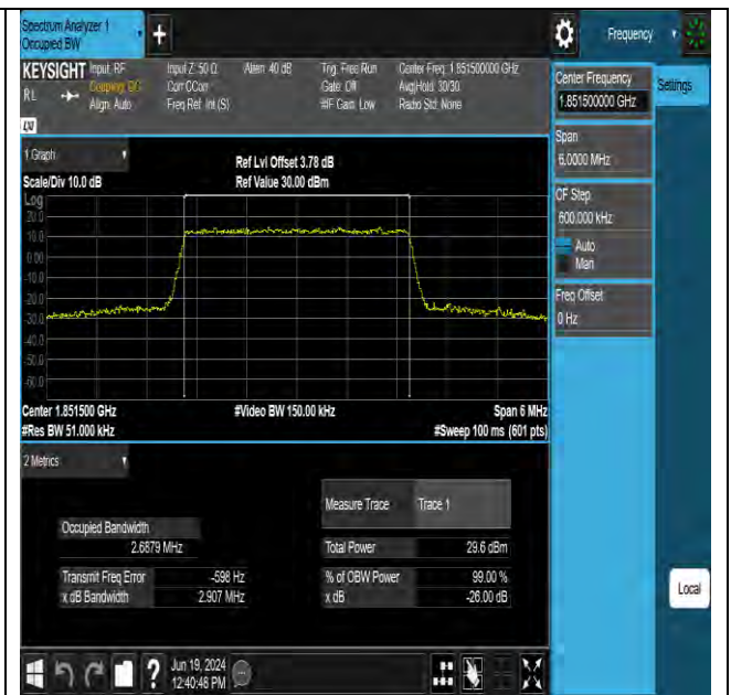
Band2-3MHz-16QAM-18615-15RB#0-PASS
