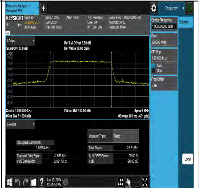
Band2-3MHz-16QAM-19185-15RB#0-PASS
