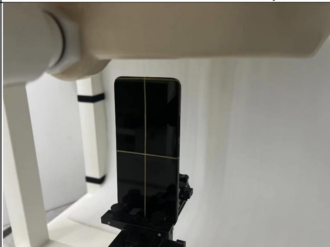
Top Side of EUT with 1.8 cm Gap
