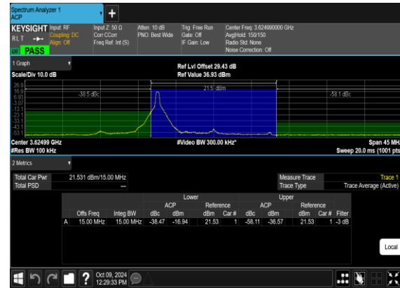
N48(15M)_DFT-s-OFDM_PI_2- BPSK_Edge_1RB_Left_Mid_CH
