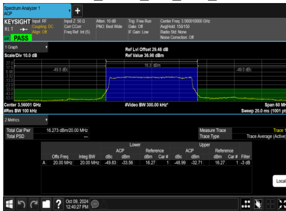
N48(20M)_DFT-s-OFDM_PI_2- BPSK_Outer_Full_Low_CH
