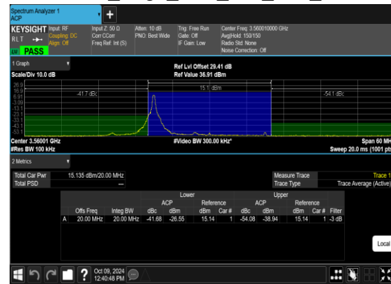
N48(20M)_DFT-s-OFDM_PI_2- BPSK_Edge_1RB_Left_Low_CH
