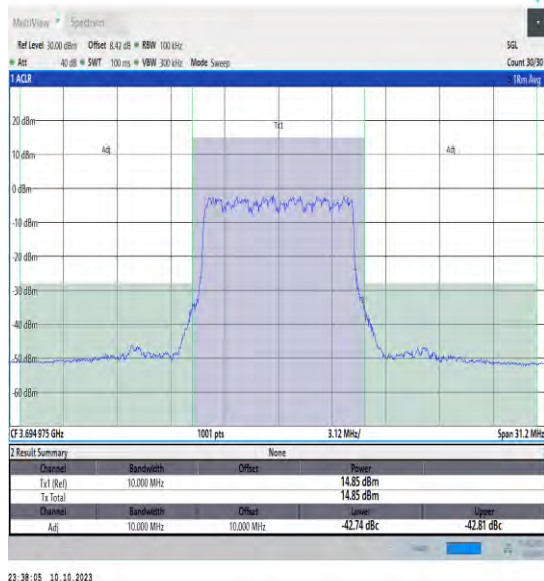
NTVN_N48_PC3_30_10_H_TID1_#1_-10_10
