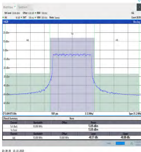
NTVN_N48_PC3_30_10_H_TID16_#1_-10_10
