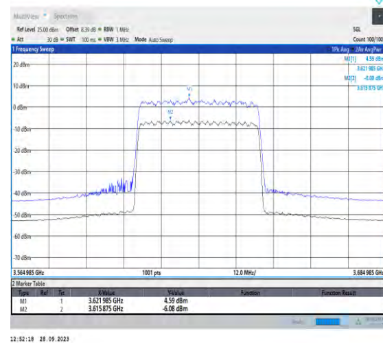
1-N48-PC3-30-40-M-2-CP-256QAM-Outer_Full-106 @0-Ant7-10.67-100%-0.00-10.67-PASS-≤13
