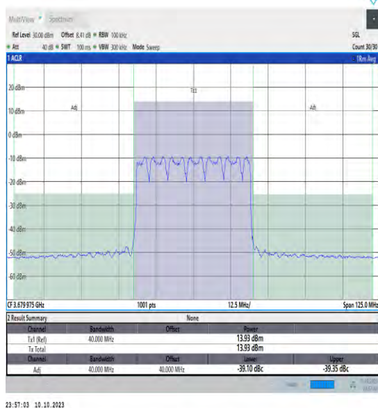
NTNV_N48_PC3_30_40_H_TID16_#1_-40_40
