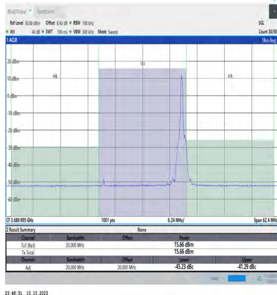
NTVN_N48_PC3_30_20_H_TID3_#1_-20_20
