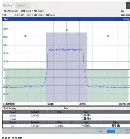
NTVN_N48_PC3_30_15_H_TID1_#1_-15_15
