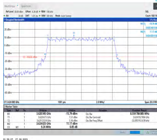
1-N48-PC3-30-10-M-4-DFT-64QAM-Outer_Full-24@0-Ant7-8.56-9.240-≤10-PASS
