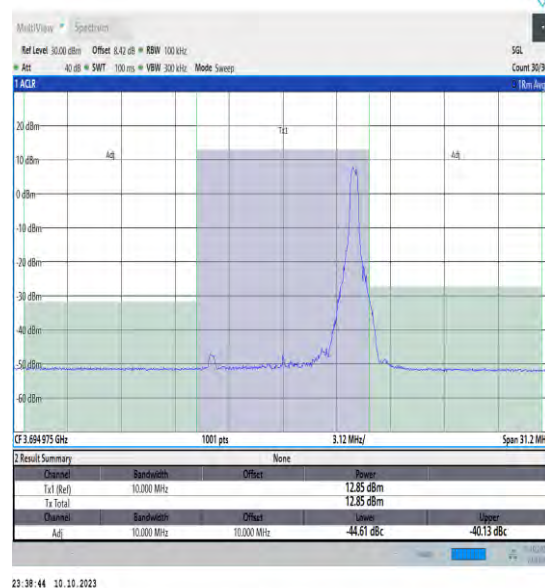
NTVN_N48_PC3_30_10_H_TID18_#1_-10_10
