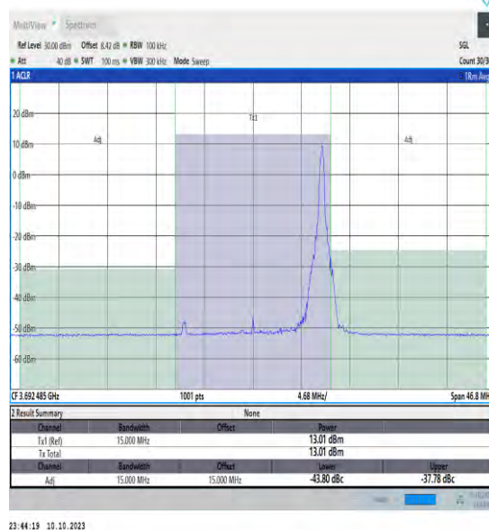
NTVN_N48_PC3_30_15_H_TID18_#1_-15_15
