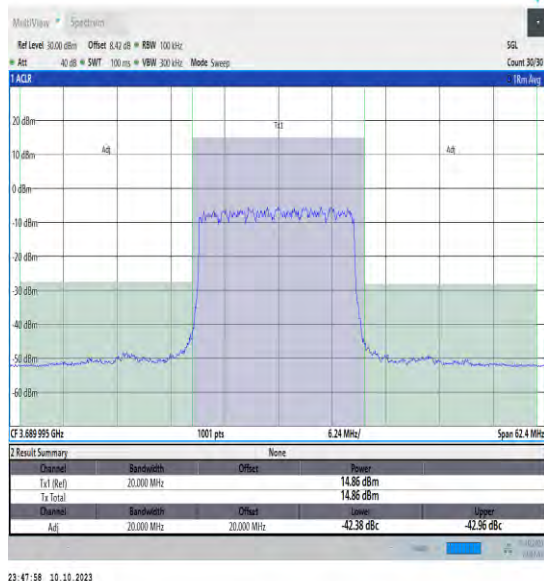
NTVN_N48_PC3_30_20_H_TID1_#1_-20_20
