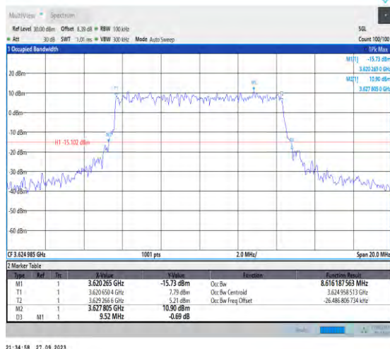
1-N48-PC3-30-10-M-3-DFT-16QAM-Outer_Full-24@0-Ant7-8.616-9.520-≤10-PASS
