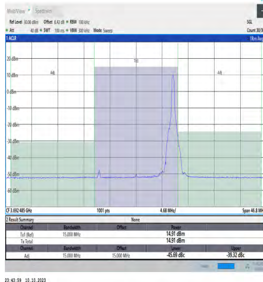
NTVN_N48_PC3_30_15_H_TID3_#1_-15_15
