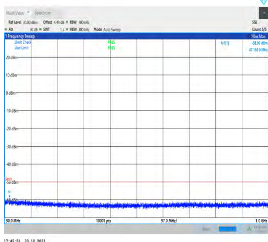
1-N48-PC3-30-40-H-1-DFT-PI2BPSK-Inner_1RB_L eft-1@1-30-1000-Ant7-61.62--54.53--50-PASS
