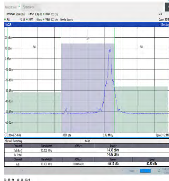
NTVN_N48_PC3_30_10_H_TID3_#1_-10_10
