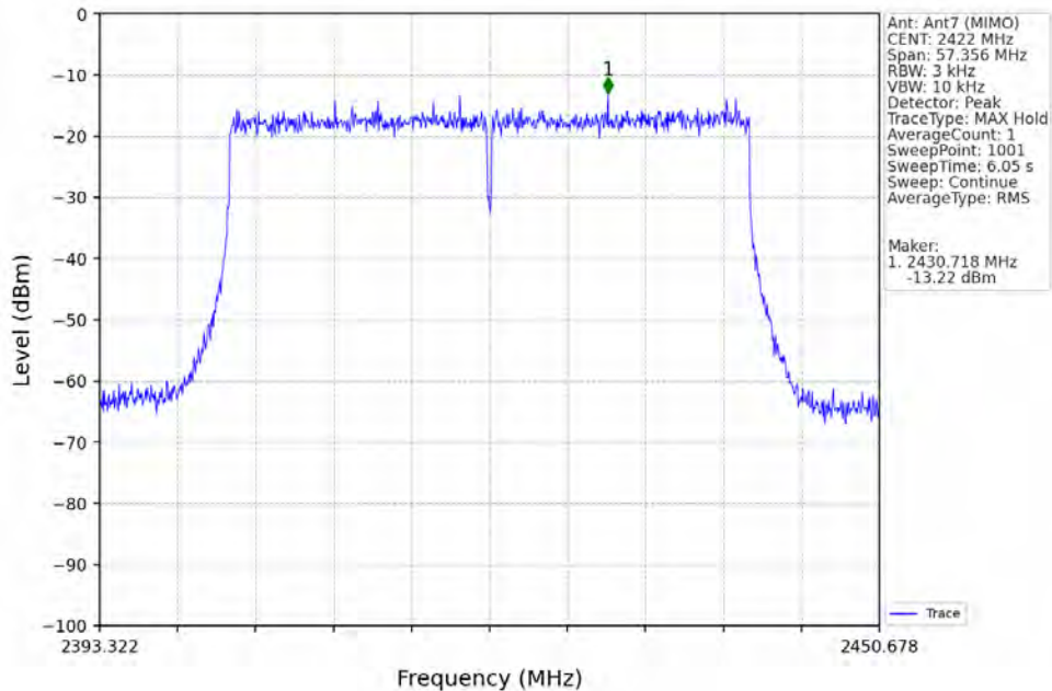
802.11ax(HEW40)_LCH_2422MHz_RU484_Left_MIMO_NTNV
