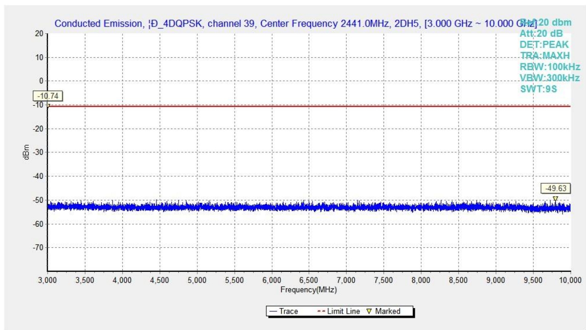
Fig.45. Conducted spurious emission: \pi/4 DQPSK, Channel 39, 3GHz - 10GHz
