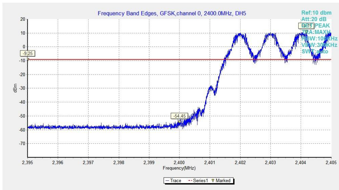
Fig.11. Frequency Band Edges: GFSK, Channel 0, Hopping On
