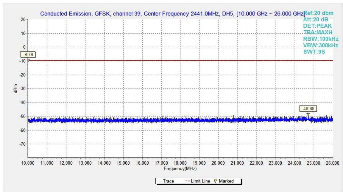
Fig.31. Conducted spurious emission: GFSK, Channel 39, 10GHz – 26GHz
