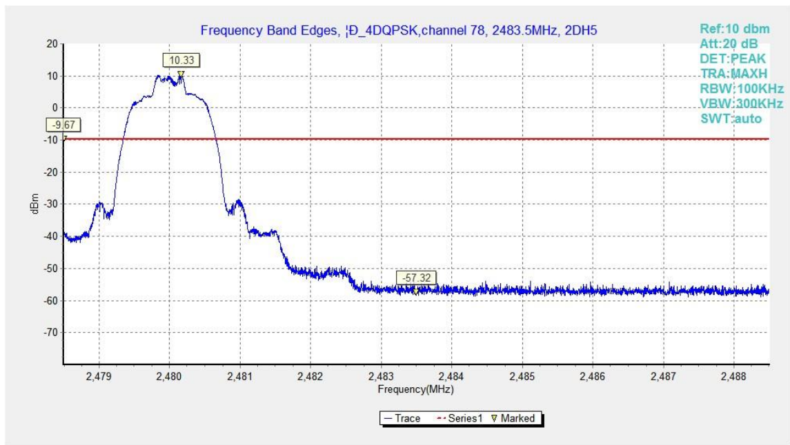
Fig.16. Frequency Band Edges: \pi/4 DQPSK, Channel 78, Hopping Off
