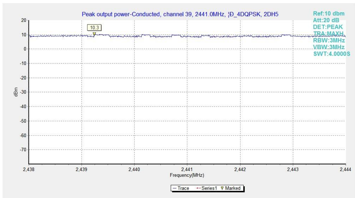
Fig.5. Peak Output Power -Conducted: \pi/4 DQPSK, Channel 39,
