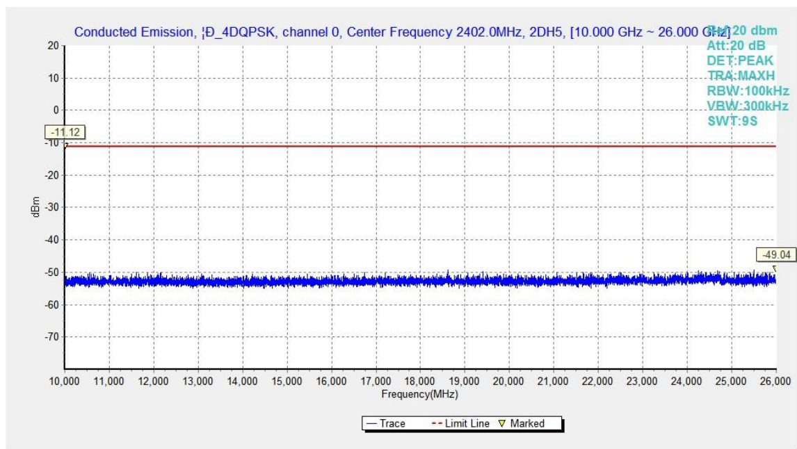
Fig.41. Conducted spurious emission: \pi/4 DQPSK, Channel 0, 10GHz - 26GHz
