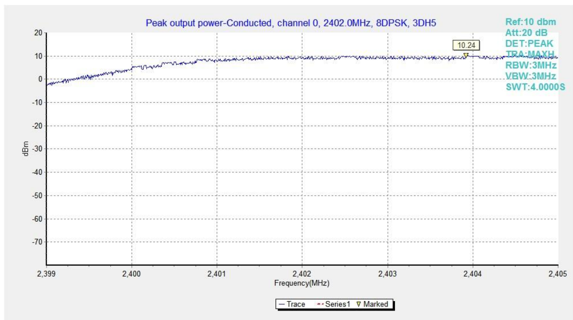
Fig.7. Peak Output Power -Conducted: 8DPSK, Channel 0,
