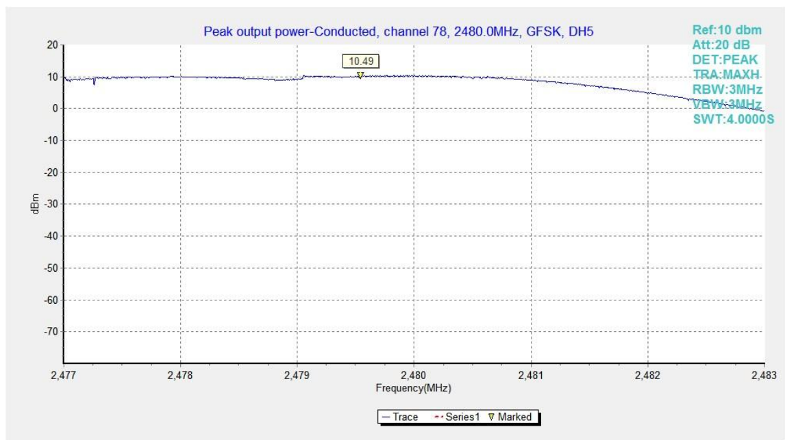
Fig.3. Peak Output Power -Conducted: GFSK, Channel 78,
