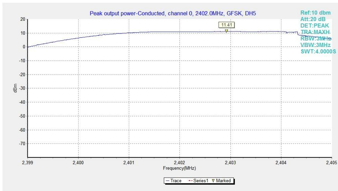
Fig.1. Peak Output Power -Conducted: GFSK, Channel 0,
