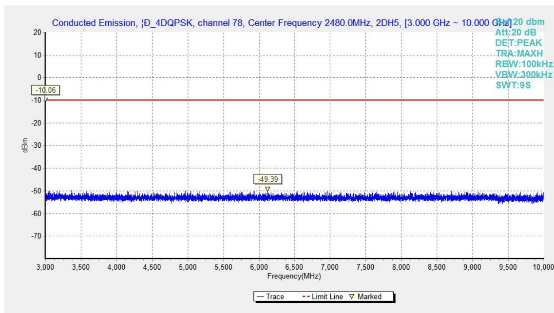
Fig.50. Conducted spurious emission: \pi/4 DQPSK, Channel 78, 3GHz - 10GHz
