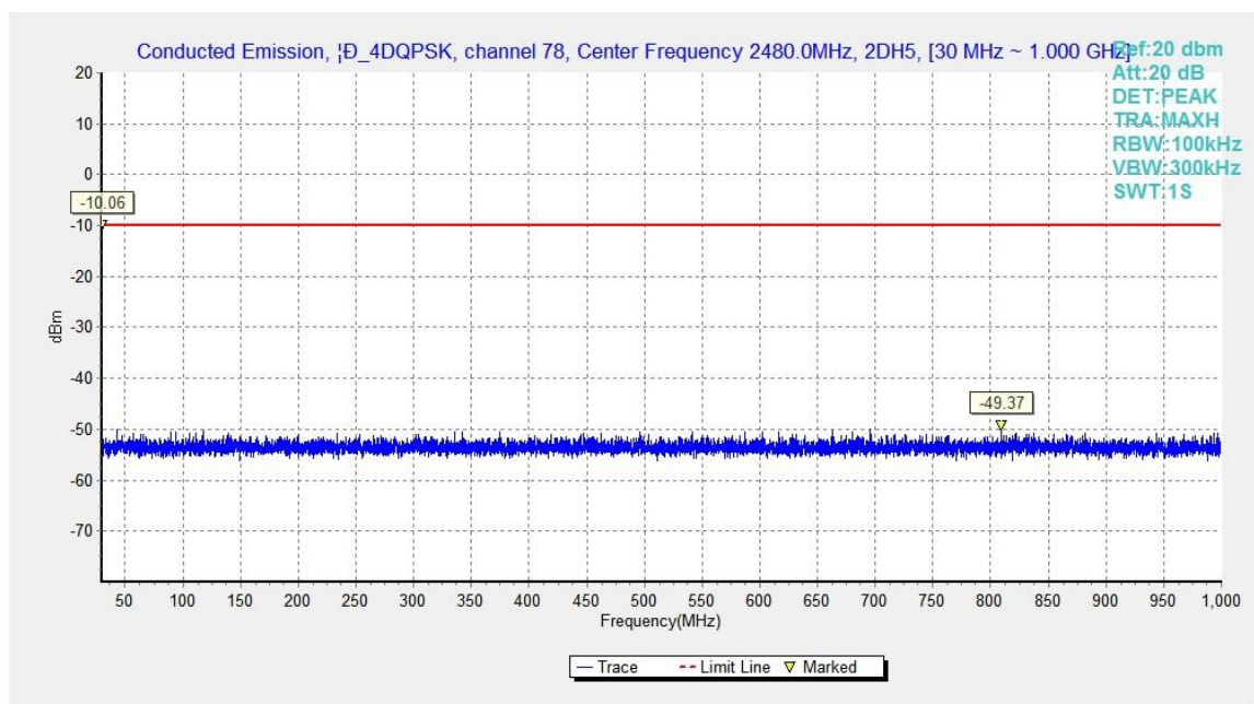
Fig.48. Conducted spurious emission: \pi/4 DQPSK, Channel 78, 30MHz - 1GHz
