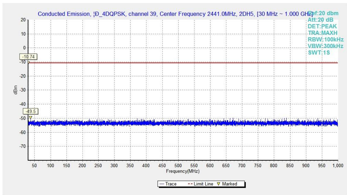
Fig.43. Conducted spurious emission: \pi/4 DQPSK, Channel 39, 30MHz - 1GHz
