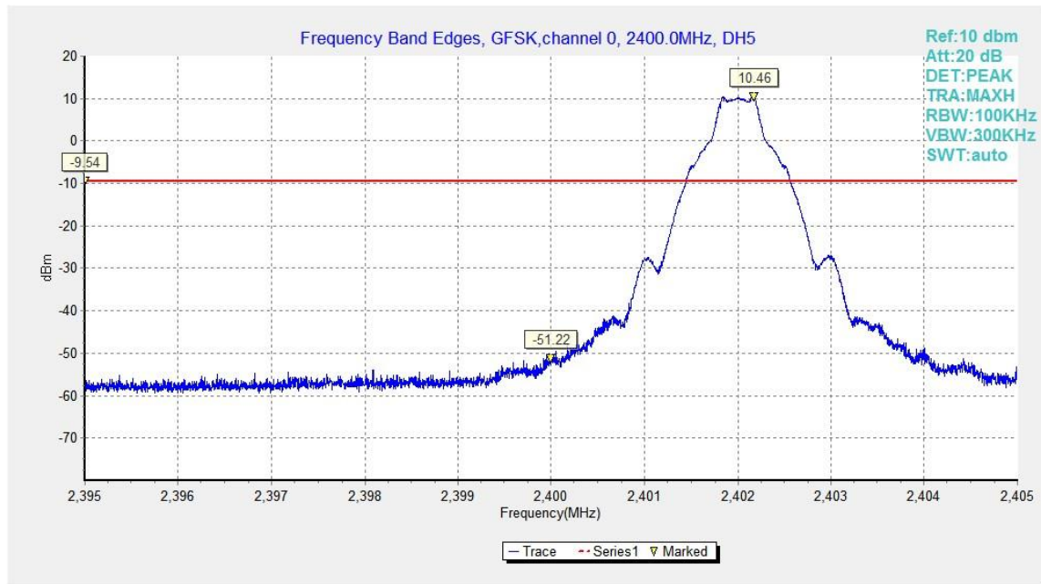
Fig.10. Frequency Band Edges: GFSK, Channel 0, Hopping Off
