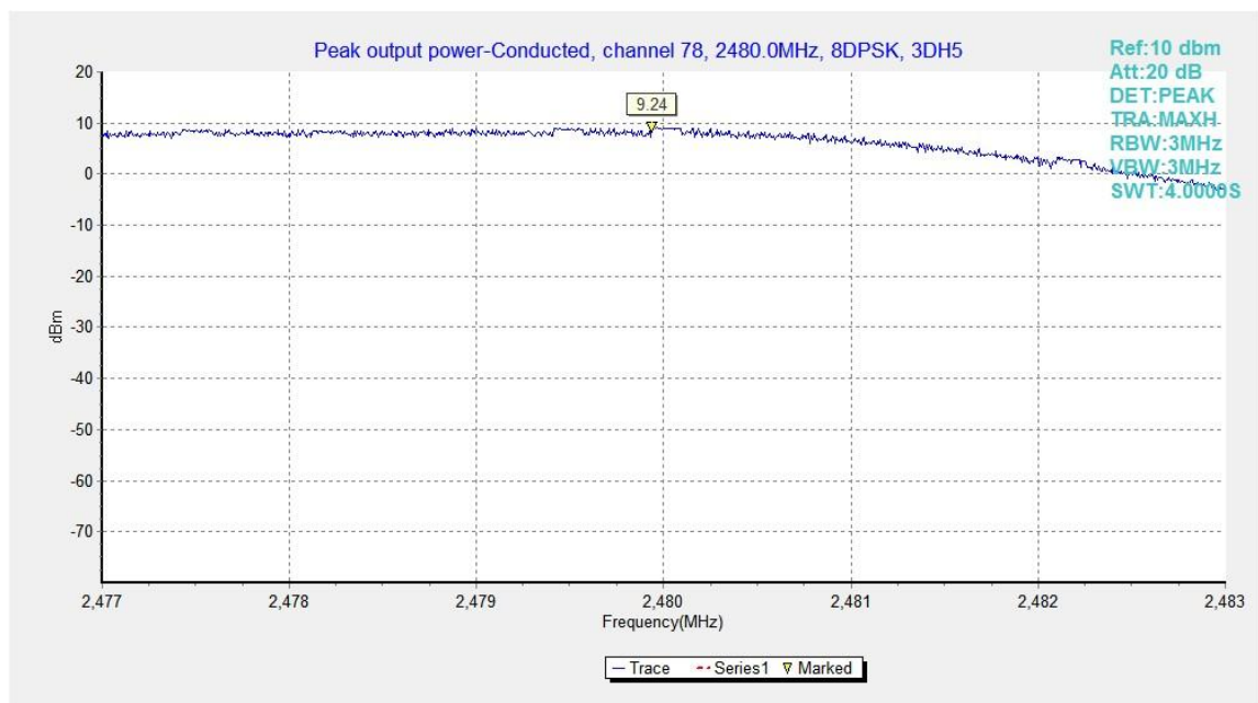
Fig.9. Peak Output Power -Conducted: 8DPSK, Channel 78,
