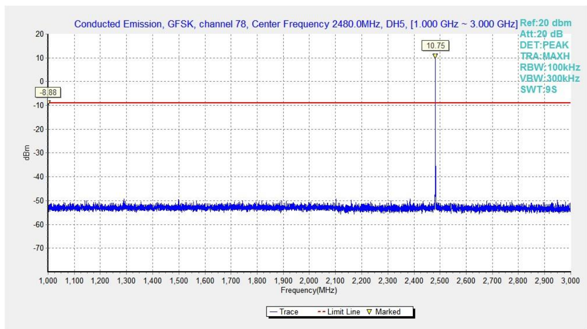
Fig.34. Conducted spurious emission: GFSK, Channel 78, 1GHz - 3GHz
