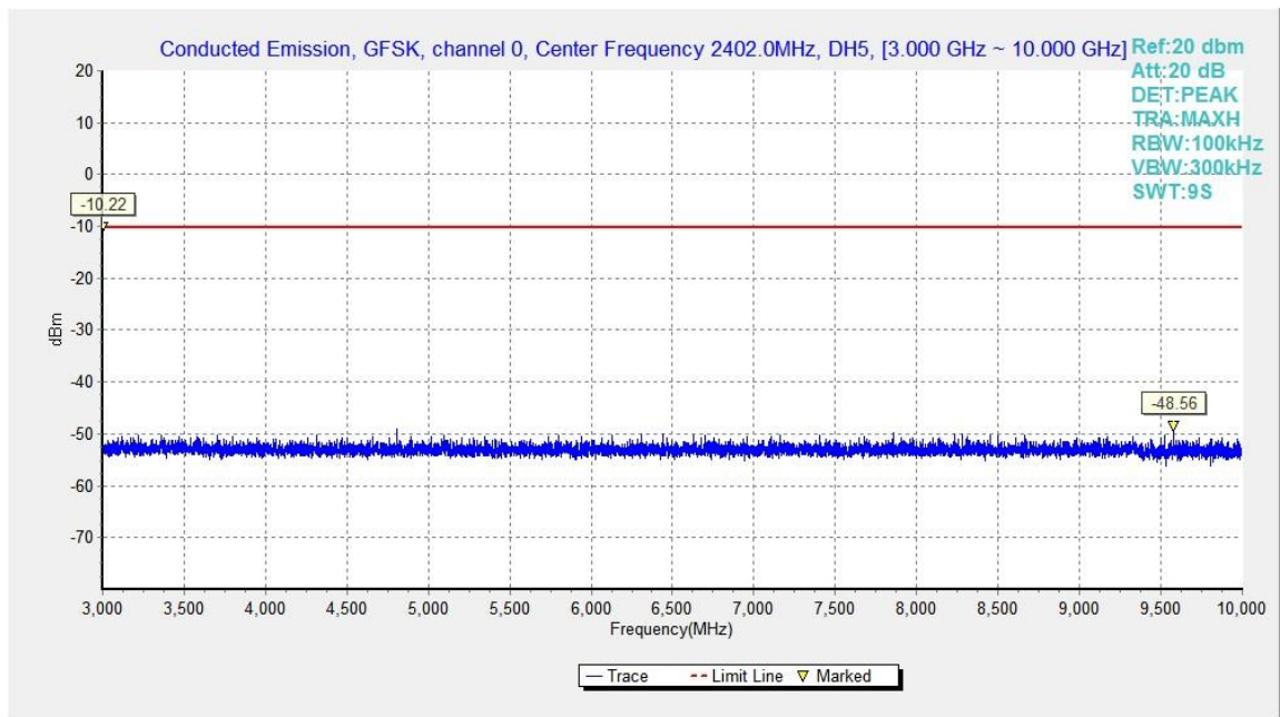
Fig.25. Conducted spurious emission: GFSK, Channel 0, 3GHz - 10GHz
