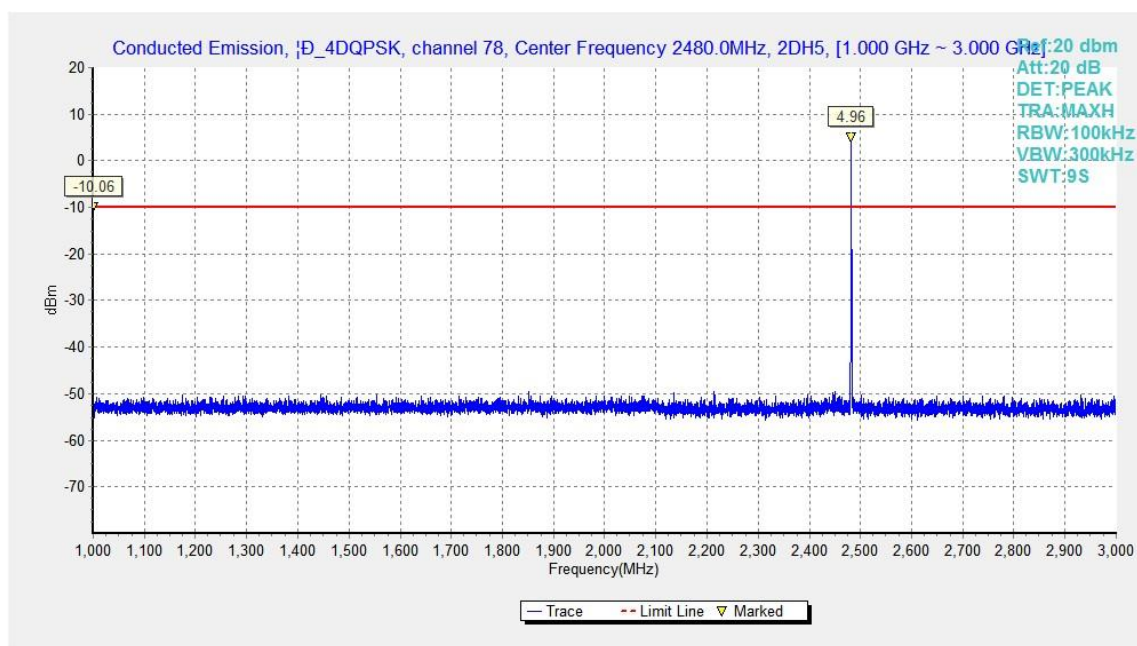
Fig.49. Conducted spurious emission: \pi/4 DQPSK, Channel 78, 1GHz - 3GHz
