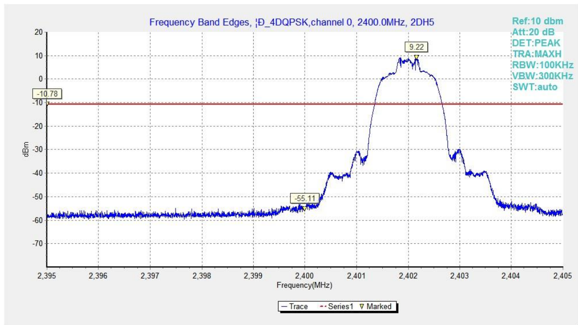
Fig.14. Frequency Band Edges: \pi/4 DQPSK, Channel 0, Hopping Off
