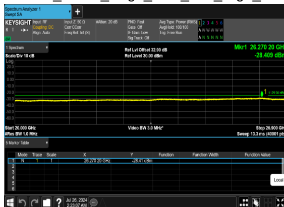
B66_N41(15M)_DFT-s-OFDM_BPSK_Edge_1RB_Left_High_CH
