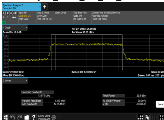
B66_N41(15M)_CP-OFDM_256 QAM_Outer_Full_Mid_CH
