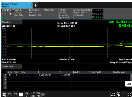
B66_N41(15M)_DFT-s-OFDM_QPSK_Edge_1RB_Left_Low_CH
