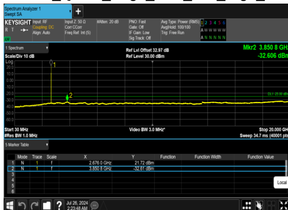
B66_N41(15M)_DFT-s-OFDM_QPSK_Edge_1RB_Left_High_CH
