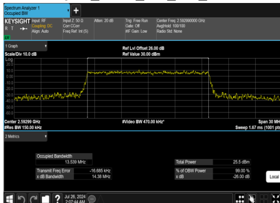
B66_N41(15M)_CP-OFDM_16 QAM_Outer_Full_Mid_CH
