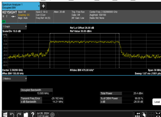
B66_N41(15M)_CP- OFDM_QPSK_Outer_Full_Mid_CH
