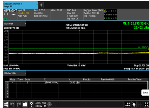
B66_N7(20M)_DFT-s- OFDM_BPSK_Edge_1RB_Left_Low_CH
