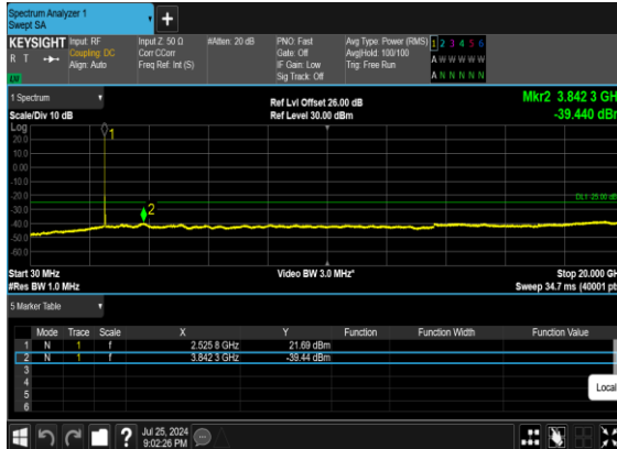
B66_N7(20M)_DFT-s- OFDM_QPSK_Edge_1RB_Left_Mid_CH
