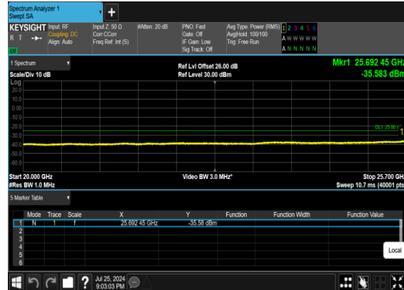
B66_N7(20M)_DFT-s- OFDM_QPSK_Edge_1RB_Left_Mid_CH
