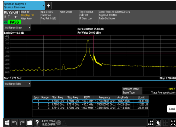
B7_N66(40M)_DFT-s- OFDM_QPSK_Edge_1RB_Right_High_CH
