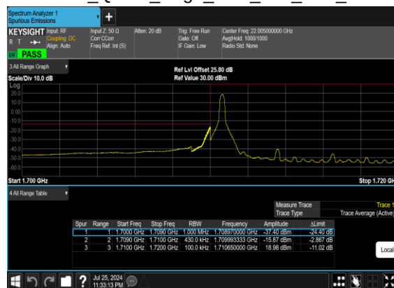
B7_N66(40M)_DFT-s- OFDM_QPSK_Edge_1RB_Left_Low_CH
