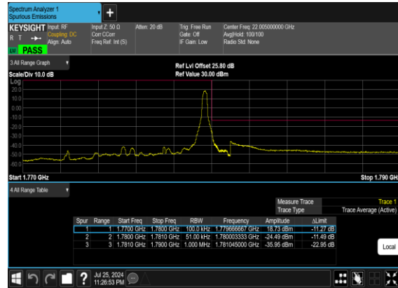
B7_N66(5M)_DFT-s-OFDM_QPSK_Edge_1RB_Right_High_CH
