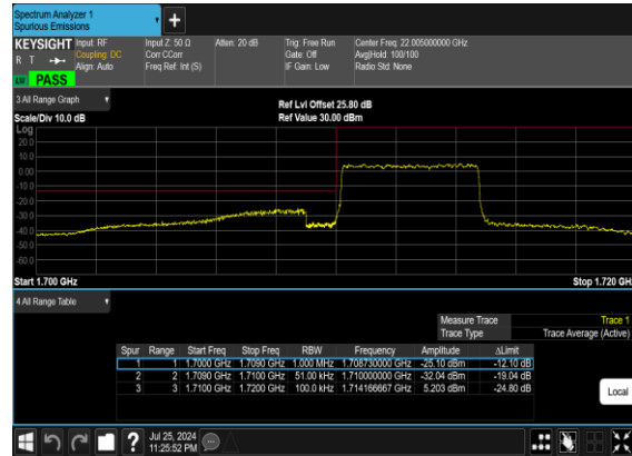
B7_N66(5M)_DFT-s- OFDM_QPSK_Outer_Full_Low_CH
