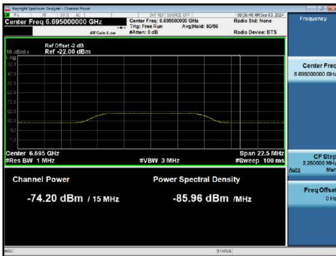
802.11ax (HE20)-Channel 149
