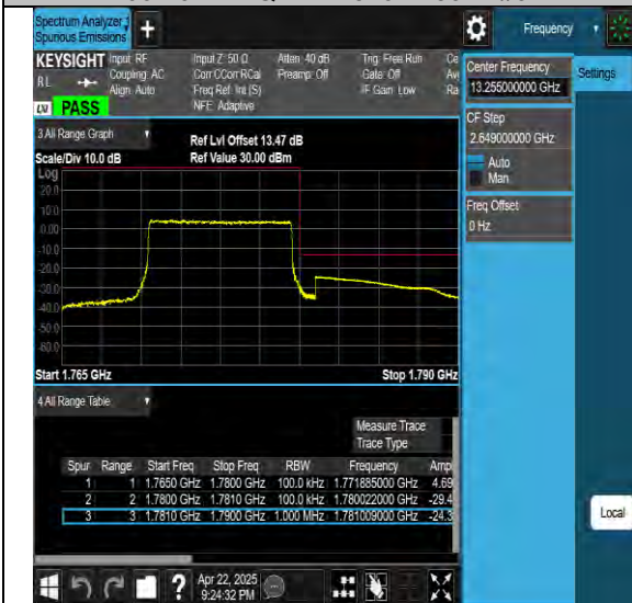
Band66-10MHz-64QAM-132022-50RB#0-PASS
