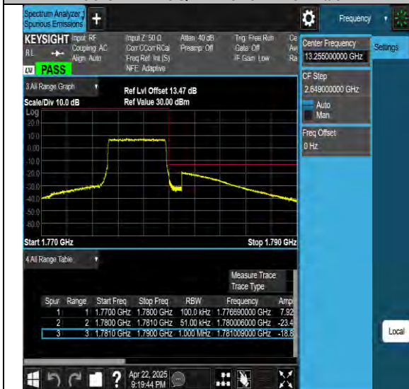
Band66-10MHz-QPSK-132022-50RB#0-PASS
