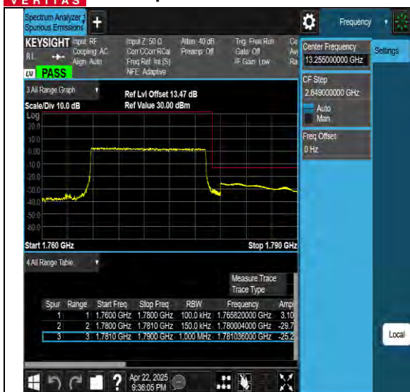
Band66-15MHz-16QAM-132047-75RB#0-PASS
