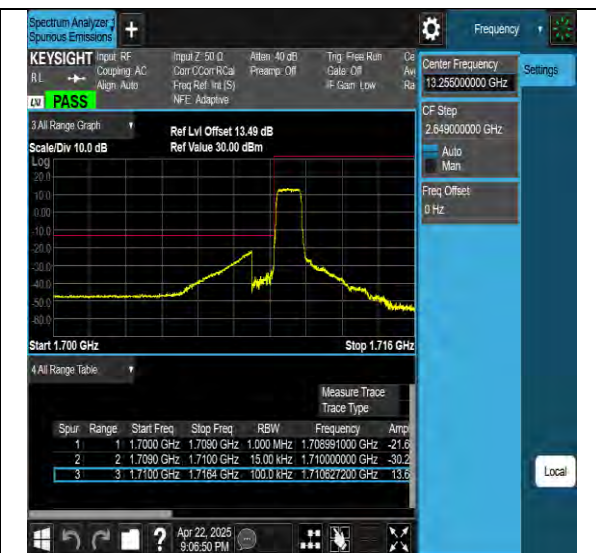
Band66-1.4MHz-64QAM-132665-6RB#0-PASS
