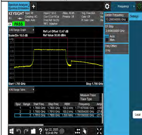
Band66-15MHz-QPSK-132047-75RB#0-PASS
