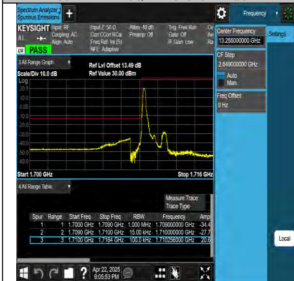
Band66-1.4MHz-16QAM-132665-1RB#5-PASS
