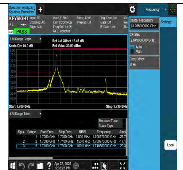
Band66-15MHz-16QAM-132597-1RB#74-PASS
