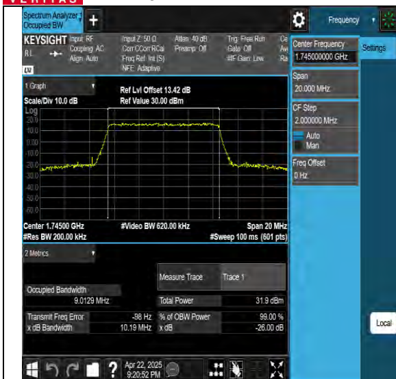
Band66-10MHz-64QAM-132022-50RB#0-PASS
