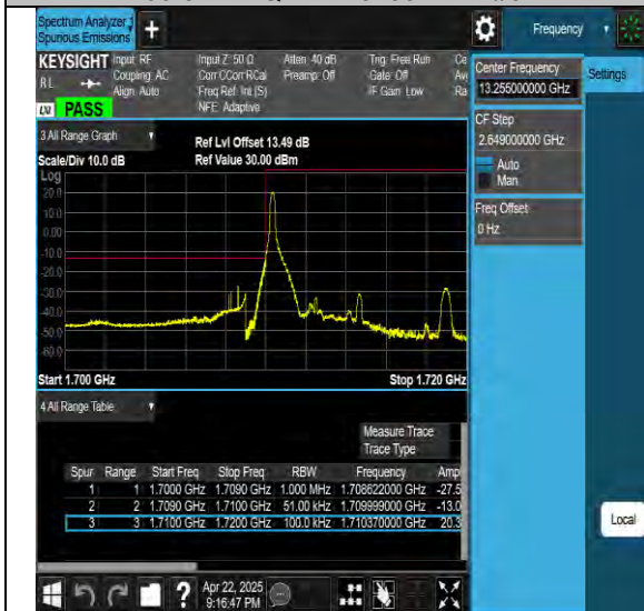
Band66-5MHz-QPSK-132647-1RB#24-PASS
