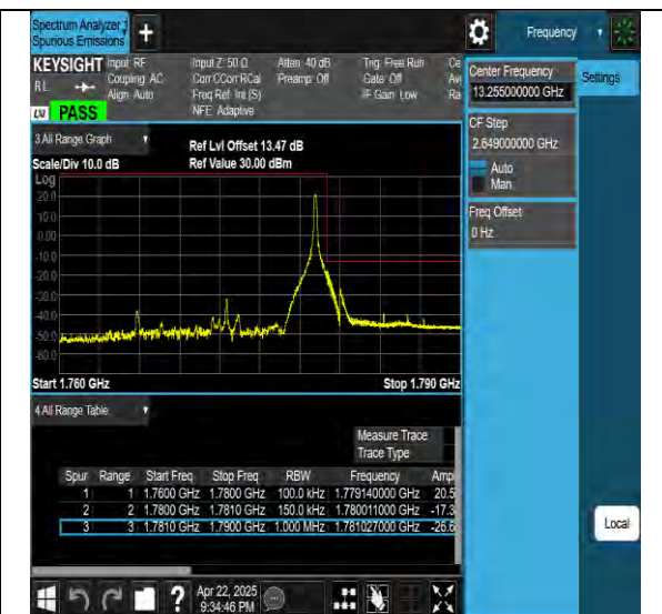
Band66-15MHz-64QAM-132047-1RB#0-PASS
