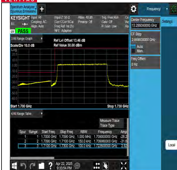
Band66-15MHz-QPSK-132597-75RB#0-PASS
