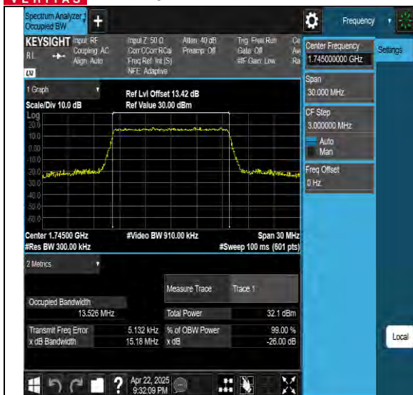
Band66-15MHz-16QAM-132047-75RB#0-PASS
