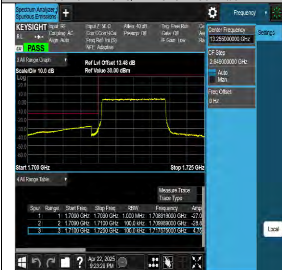
Band66-10MHz-64QAM-132622-50RB#0-PASS
