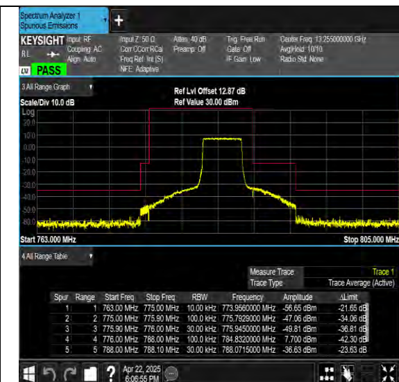
Band13-10MHz-QPSK-23230-1RB#49-PASS
