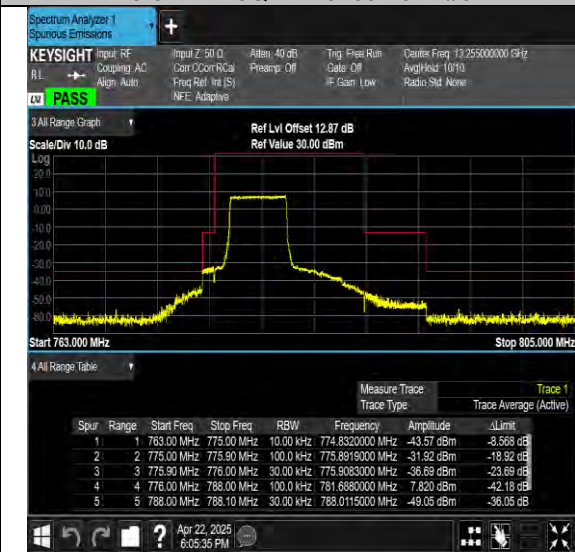
Band13-5MHz-16QAM-23255-25RB#0-PASS
