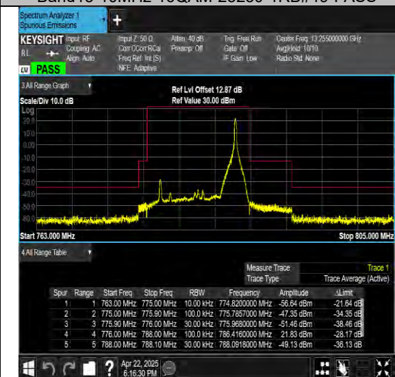
Band13-10MHz-16QAM-23230-1RB#49-PASS
