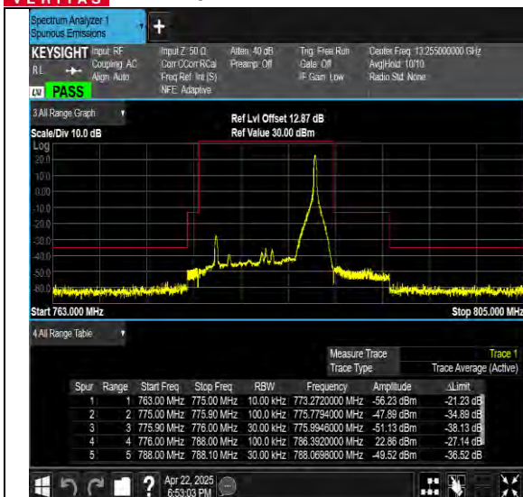
Band13-10MHz-16QAM-23230-1RB#0-PASS
