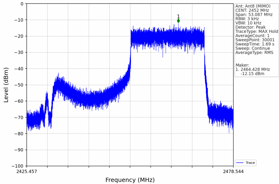
802.11ax(HEW40)_HCH_2452MHz_RU242_Right_MIMO_NTNV
