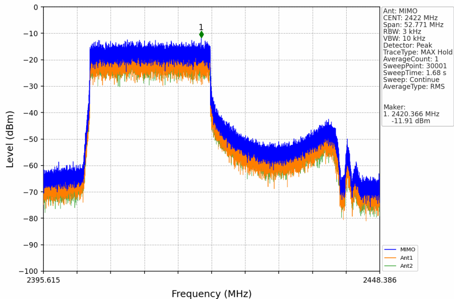
802.11ax(HEW40)_LCH_2422MHz_RU242_Left_MIMO_NTNV
