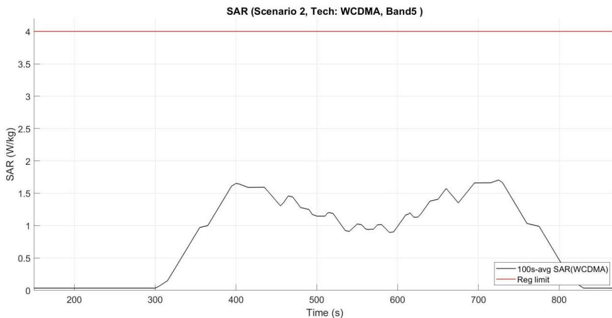
Figure 5- 17 Time-averaged SAR
