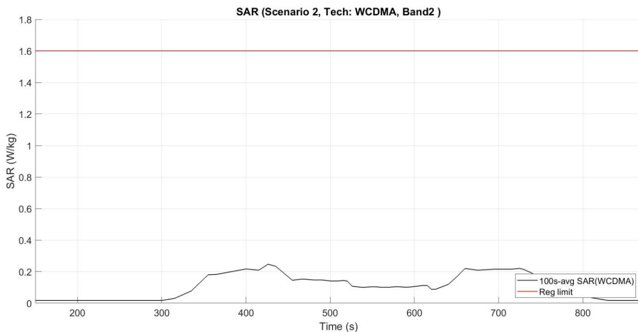
Figure 5- 21 Time-averaged SAR
