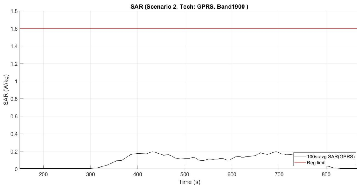
Figure 5- 10 Time-averaged SAR
