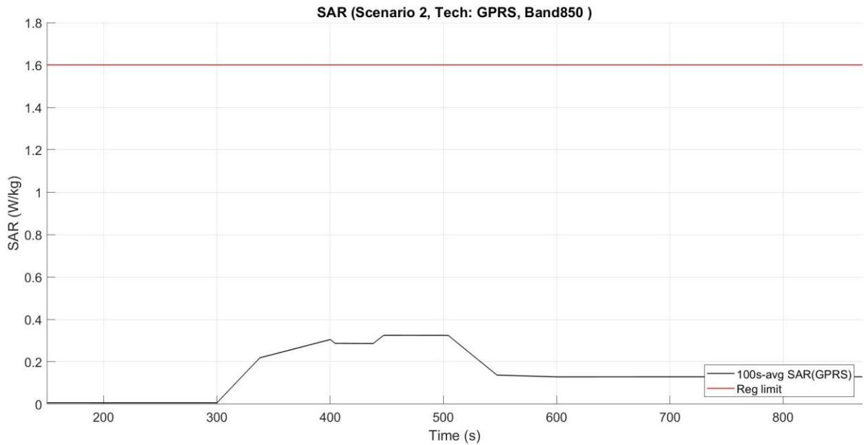
Figure 5- 12 Time-averaged SAR
