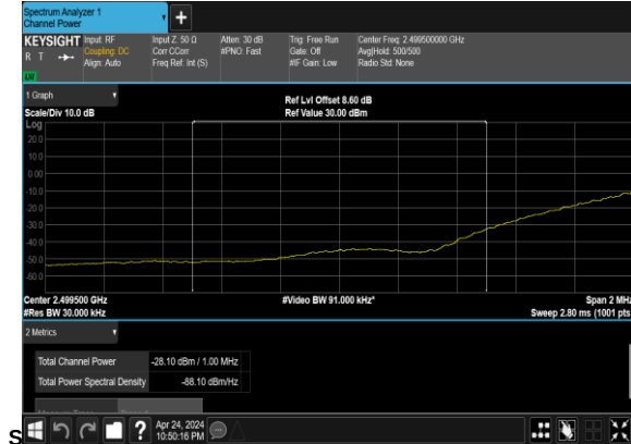
N7(50M)_DFT-s- OFDM_BPSK_Edge_1RB_Left_Low_CH_CHP_PAS
