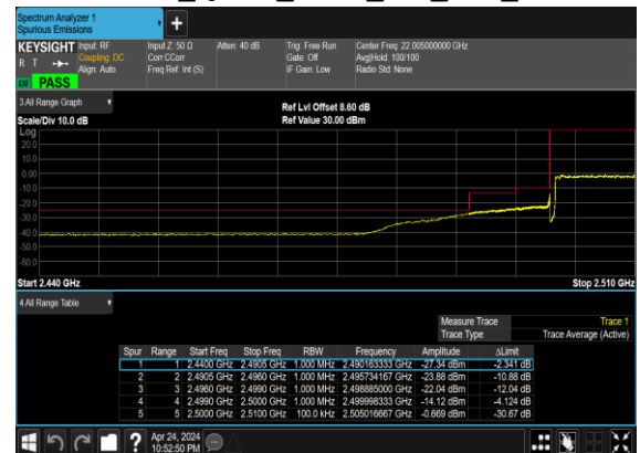
N7(50M)_DFT-s- OFDM_QPSK_Outer_Full_Low_CH
