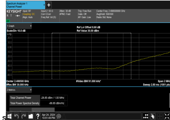
N7(50M)_DFT-s- OFDM_QPSK_Edge_1RB_Left_Low_CH_CHP_PAS
