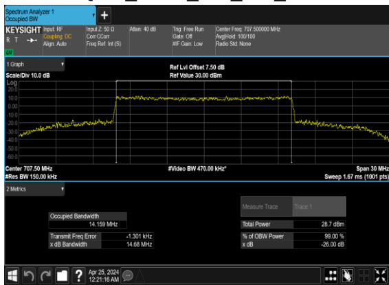
N12(15M)_CP-OFDM_16 QAM_Outer_Full_Mid_CH
