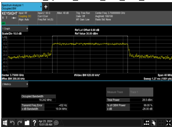
N78(20M)_CP- OFDM_QPSK_Outer_Full_Mid_CH
