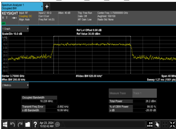
N78(20M)_CP-OFDM_64 QAM_Outer_Full_Mid_CH
