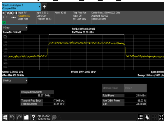
N78(40M)_CP-OFDM_256 QAM_Outer_Full_Mid_CH
