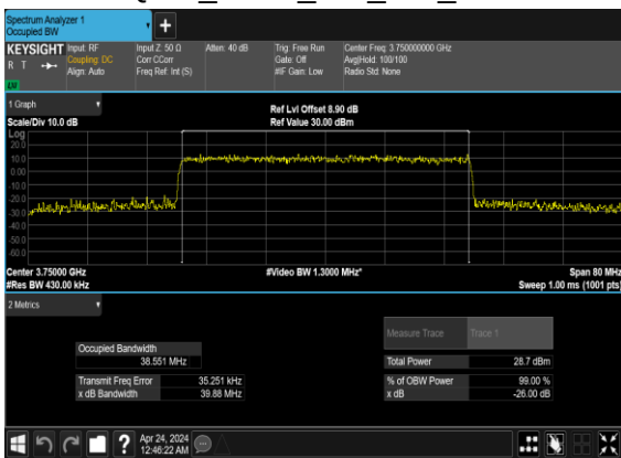
N78(40M)_CP-OFDM_64 QAM_Outer_Full_Mid_CH
