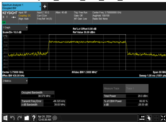
N78(40M)_CP-OFDM_16 QAM_Outer_Full_Mid_CH
