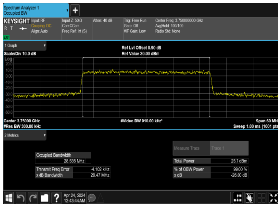
N78(30M)_CP-OFDM_256 QAM_Outer_Full_Mid_CH
