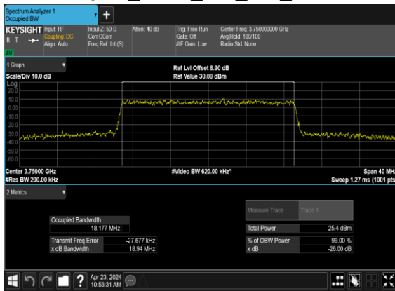
N78(20M)_CP-OFDM_256 QAM_Outer_Full_Mid_CH
