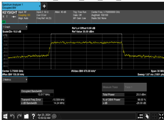
N78(15M)_CP-OFDM_256 QAM_Outer_Full_Mid_CH
