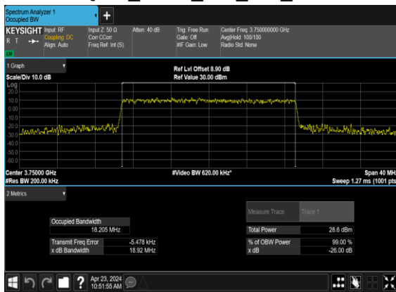
N78(20M)_CP-OFDM_16 QAM_Outer_Full_Mid_CH
