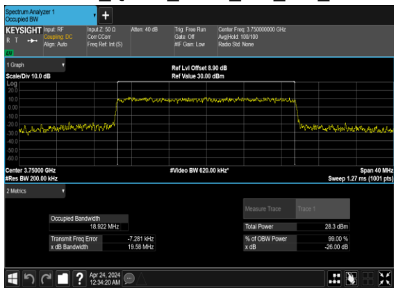
N78(20M)_CP- OFDM_QPSK_Outer_Full_Mid_CH
