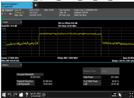
N78(40M)_CP- OFDM_QPSK_Outer_Full_Mid_CH
