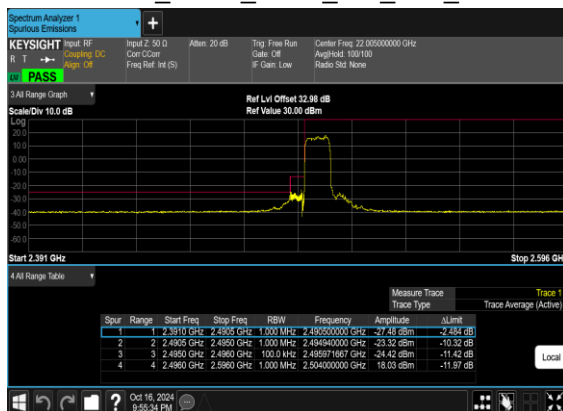
B66_N41(10M)_DFT-s- OFDM_BPSK_Outer_Full_Low_CH
