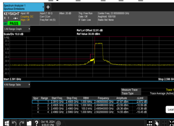
B66_N41(10M)_DFT-s- OFDM_QPSK_Outer_Full_Low_CH
