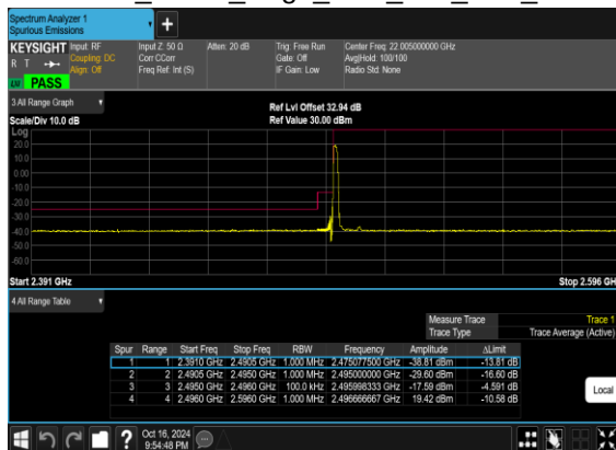
B66_N41(10M)_DFT-s- OFDM_BPSK_Edge_1RB_Left_Low_CH
