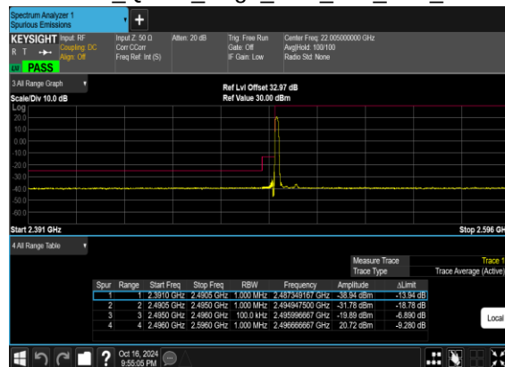
B66_N41(10M)_DFT-s- OFDM_QPSK_Edge_1RB_Left_Low_CH
