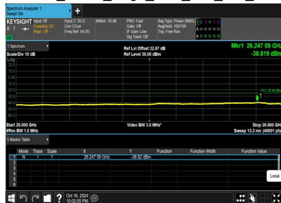
B66_N41(10M)_DFT-s-OFDM_BPSK_Edge_1RB_Left_Mid_CH
