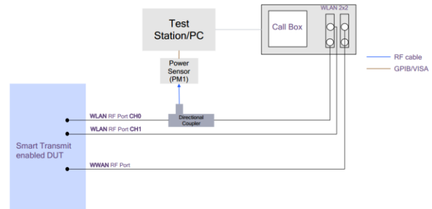
WLAN DBS Test setup - MIMO
