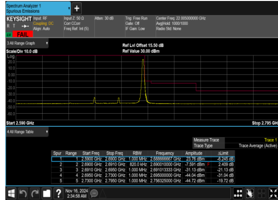
N41(40M)_DFT-s- OFDM_BPSK_Edge_1RB_Right_High_CH
