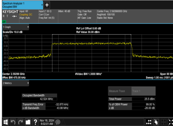
N41(45M)_CP- OFDM_QPSK_Outer_Full_Mid_CH
