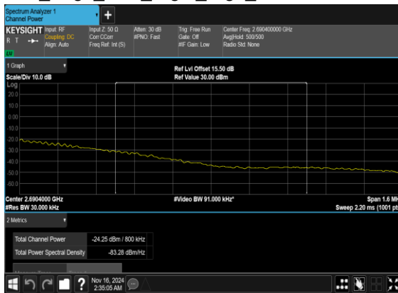
N41(40M)_DFT-s-OFDM_BPSK _Edge_1RB_Right_High_CH_CHP_PASS
