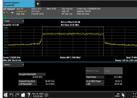
N41(35M)_CP-OFDM_16 QAM_Outer_Full_Mid_CH
