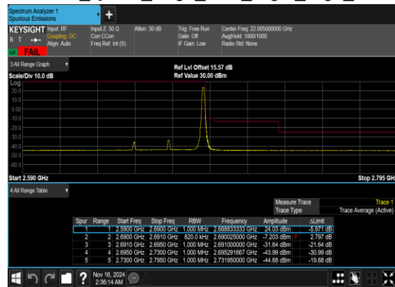
N41(40M)_DFT-s- OFDM_QPSK_Edge_1RB_Right_High_CH
