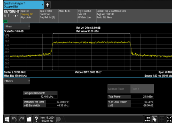
N41(45M)_CP-OFDM_16 QAM_Outer_Full_Mid_CH
