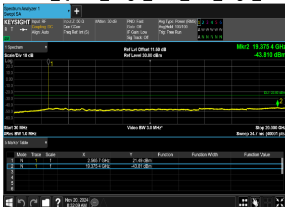
N7(5M)_CP- OFDM_QPSK_Edge_1RB_Left_High_CH
