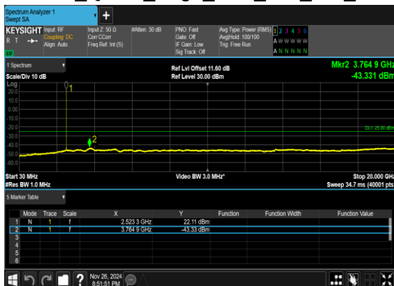
N7(25M)_CP- OFDM_QPSK_Edge_1RB_Left_Mid_CH
