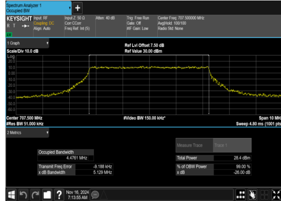
N12(5M)_CP-OFDM_16 QAM_Outer_Full_Mid_CH
