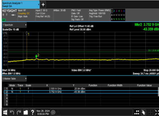
N7(50M)_CP- OFDM_QPSK_Edge_1RB_Left_Low_CH
