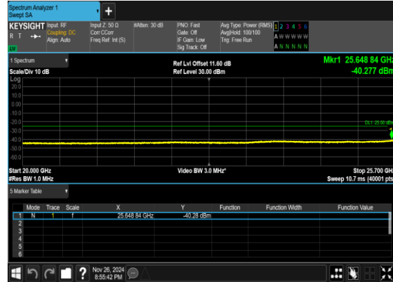
N7(50M)_CP- OFDM_QPSK_Edge_1RB_Left_Low_CH
