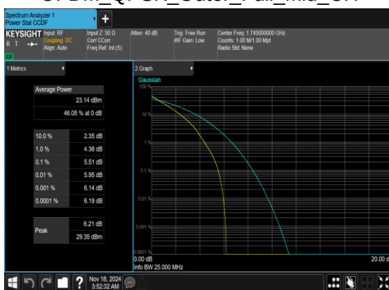
N66(20M)_DFT-s-OFDM_QPSK_Outer_Full_Mid_CH
