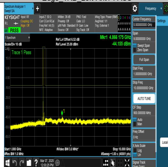
NTNV-N77-3450-3550-PC2-30-90-L-DFT-QPSK-
