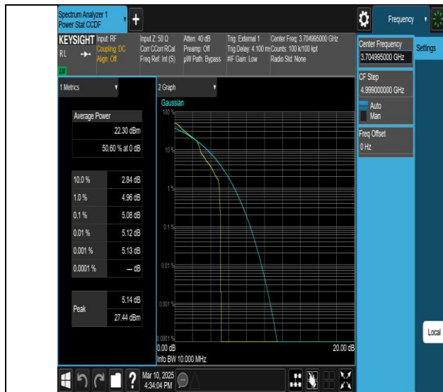
NTNV-N77-3700-3980-PC2-30-10-L-DFT-QPSK-Edge 1RB Left-PASS
