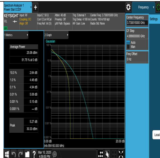
NTNV-N77-3700-3980-PC2-30-60-L-DFT-QPSK-Outer_Full-PASS
