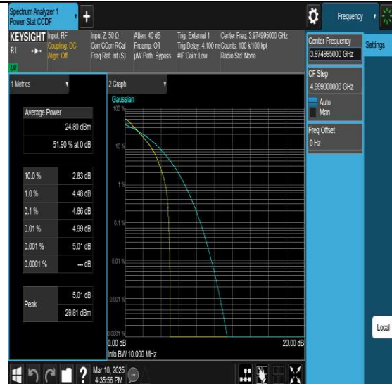
NTNV-N77-3700-3980-PC2-30-10-H-DFT-QPSK-Outer_Full-PASS
