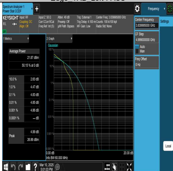
NTNV-N77-3700-3980-PC2-30-60-M-DFT-QPSK-Edge 1RB Left-PASS
