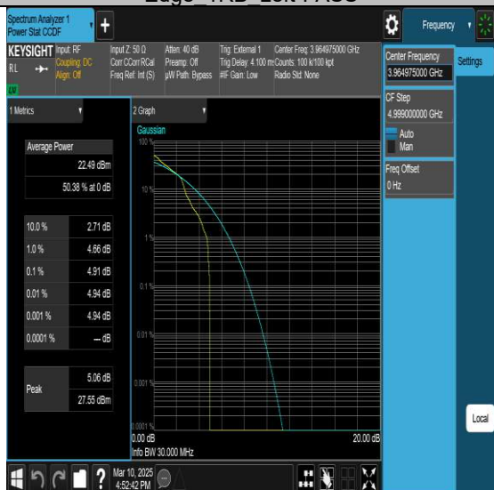
NTNV-N77-3700-3980-PC2-30-30-H-DFT-QPSK-Edge 1RB Left-PASS
