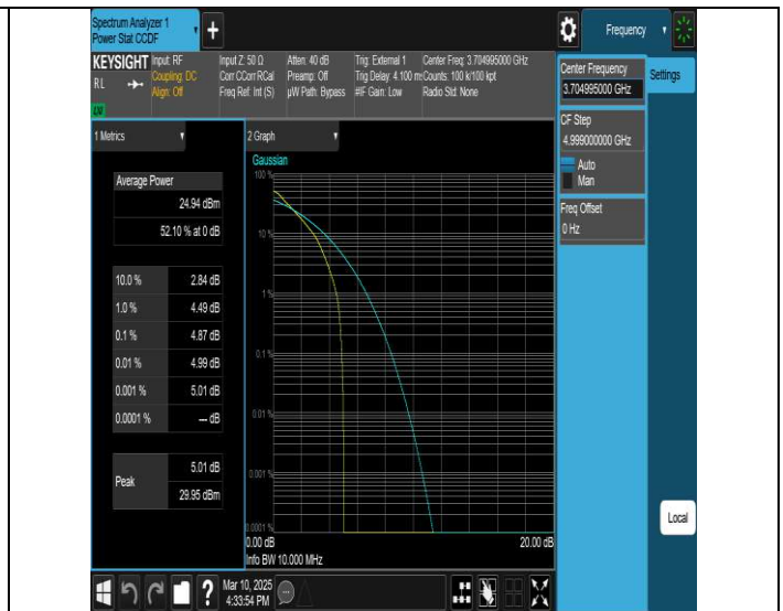
NTNV-N77-3700-3980-PC2-30-10-L-DFT-QPSK-Outer_Full-PASS
