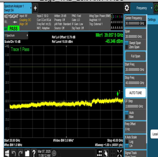
NTNV-N77-3450-3550-PC2-30-80-H-DFT-QPSK- Edge 1RB Left-Ant1-PASS
