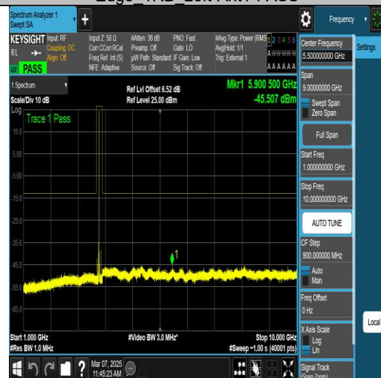
NTNV-N77-3450-3550-PC2-30-70-H-DFT-QPSK-
