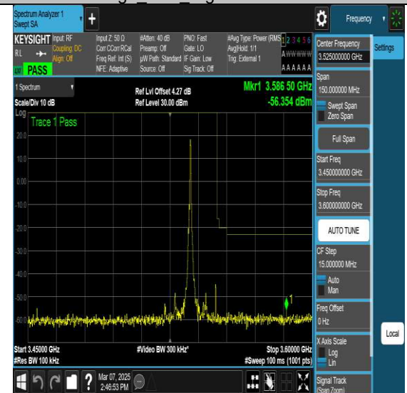
NTNV-N77-3450-3550-PC2-30-15-H-DFT-QPSK-
