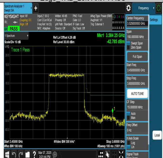
NTNV-N77-3450-3550-PC2-30-50-H-DFT-QPSK-Outer_Full-
