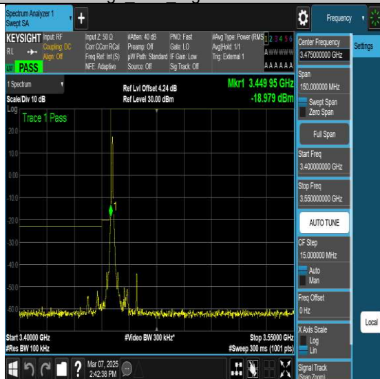
NTNV-N77-3450-3550-PC2-30-15-L-DFT-QPSK-Edge 1RB Left-Ant1-PASS
