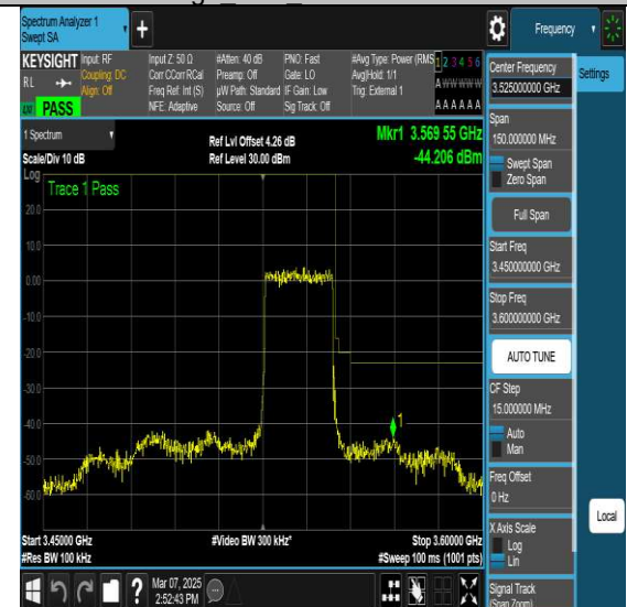
NTNV-N77-3450-3550-PC2-30-25-H-DFT-QPSK-Outer_Full-Ant1-PASS
