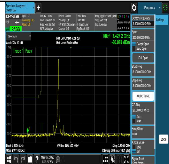
NTNV-N77-3450-3550-PC2-30-30-L-DFT-QPSK-
