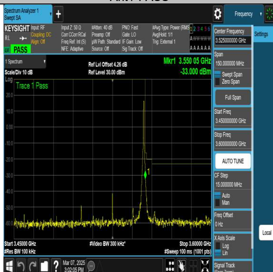
NTNV-N77-3450-3550-PC2-30-50-H-DFT-QPSK-
