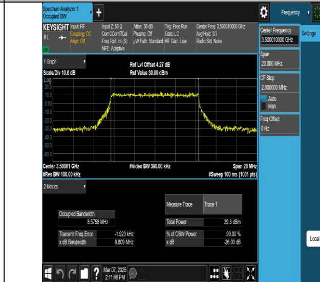
NTNV-N77-3450-3550-PC2-30-10-M-DFT-64QAM-Outer_Full-Ant1-PASS
