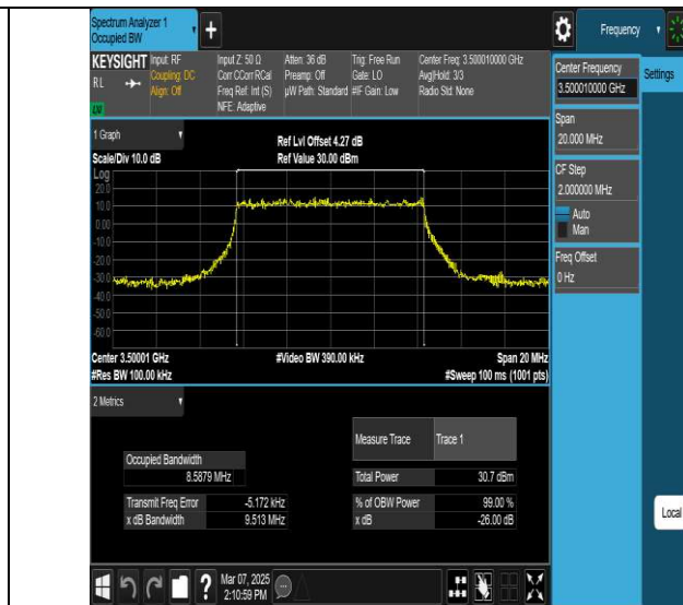
NTNV-N77-3450-3550-PC2-30-10-M-DFT-QPSK-Outer_Full-Ant1-PASS
