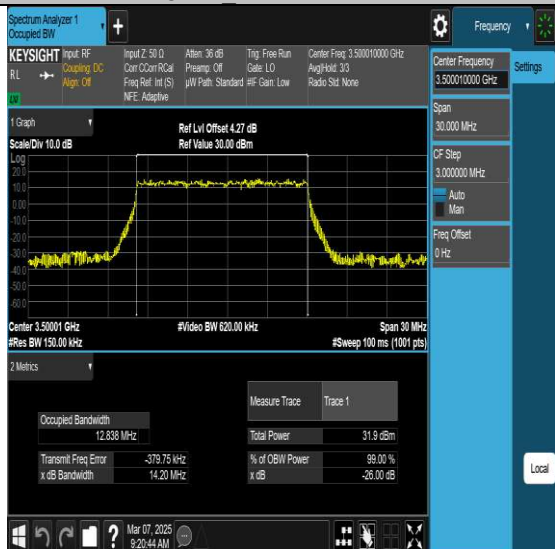
NTNV-N77-3450-3550-PC2-30-15-M-DFT-QPSK-Outer Full-Ant1-PASS
