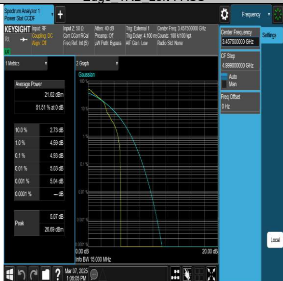
NTNV-N77-3450-3550-PC2-30-15-L-DFT-QPSK-Edge 1RB Left-PASS
