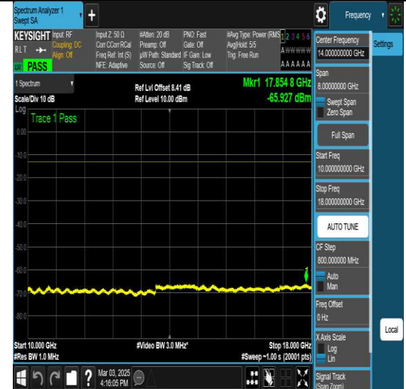
NTVN-N66-PC3-15-30-H-DFT-QPSK-Edge_1RB_Left-Ant1-PASS
