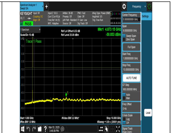
NTNV-N66-PC3-15-5-L-DFT-QPSK-Edge_1RB_Left-Ant1-PASS
