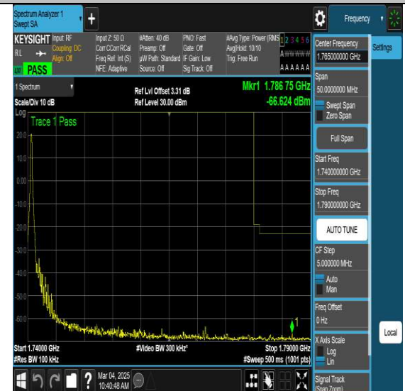
NTVN-N66-PC3-15-40-H-DFT-QPSK-Edge_1RB_Left-Ant1-PASS
