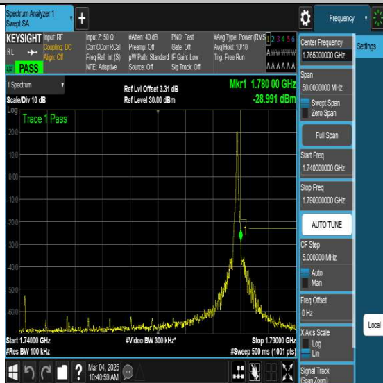
NTVN-N66-PC3-15-40-H-DFT-QPSK-Edge_1RB_Right-Ant1-PASS
