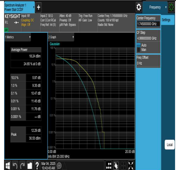
NTNV-N66-PC3-15-25-M-DFT-QPSK-Outer Full-PASS
