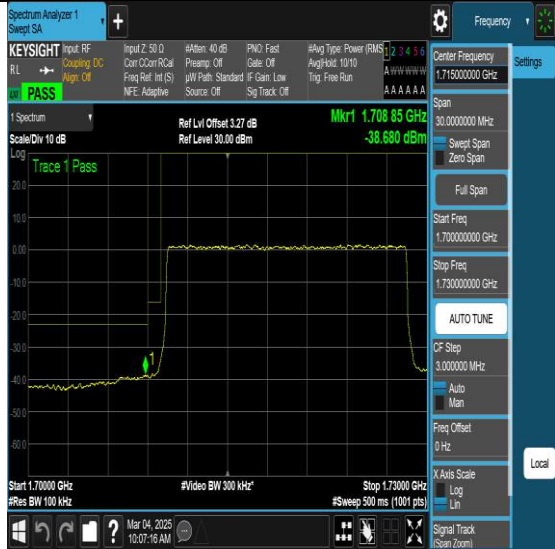
NTNV-N66-PC3-15-20-L-DFT-QPSK-Outter_Full-Ant1-PASS
