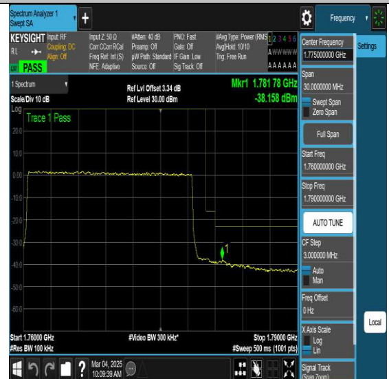
NTNV-N66-PC3-15-20-H-DFT-QPSK-Outter_Full-Ant1-PASS
