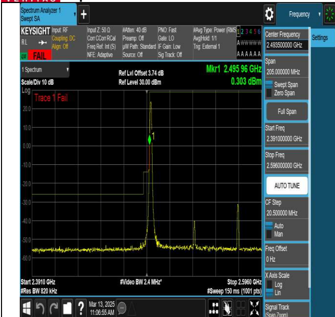
NTNV-N41-PC3-30-80-L-DFT-QPSK-Edge_1RB_Left-Ant1- FAIL
