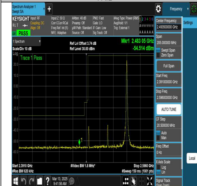
NTNV-N41-PC3-30-60-L-DFT-QPSK-Edge_1RB_Right-Ant1- PASS
