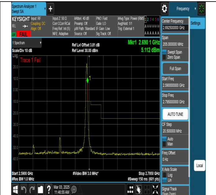
NTNV-N41-PC3-30-80-H-DFT-QPSK-Edge_1RB_Right-Ant1-FAIL
