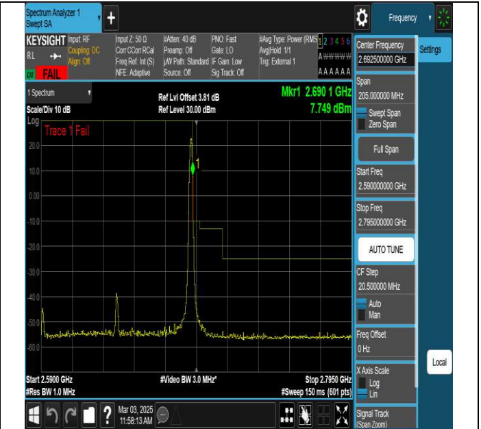
NTNV-N41-PC3-30-100-H-DFT-QPSK-Edge_1RB_Right-Ant1-FAIL
