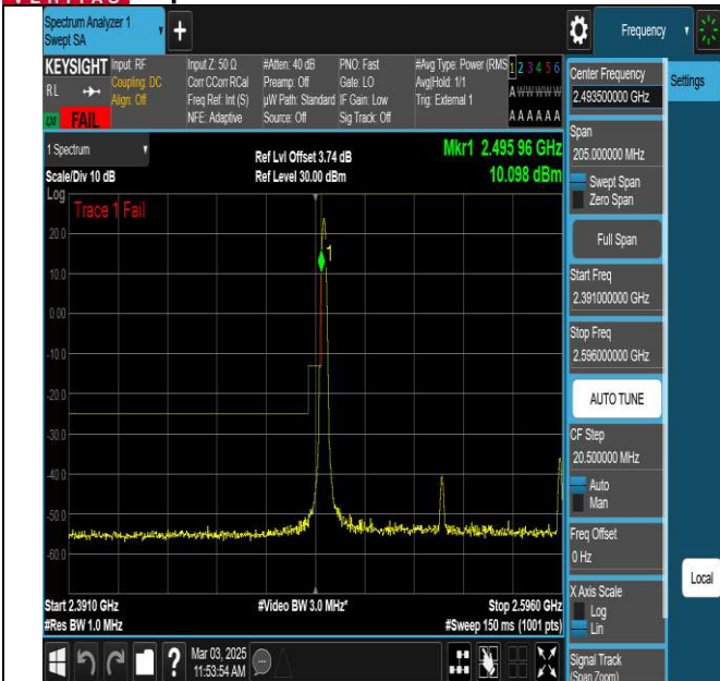
NTNV-N41-PC3-30-100-L-DFT-QPSK-Edge_1RB_Left-Ant1- FAIL
