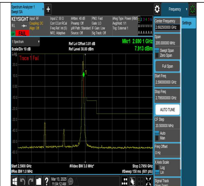
NTNV-N41-PC3-30-60-H-DFT-QPSK-Edge_1RB_Right-Ant1- FAIL
