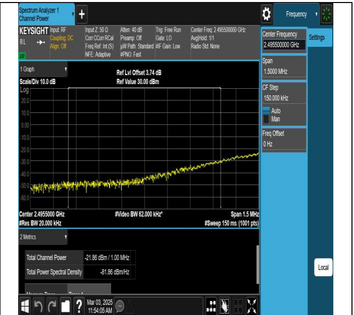
NTNV-N41-PC3-30-100-L-DFT-QPSK-Edge_1RB_Left-Ant1- PASS
