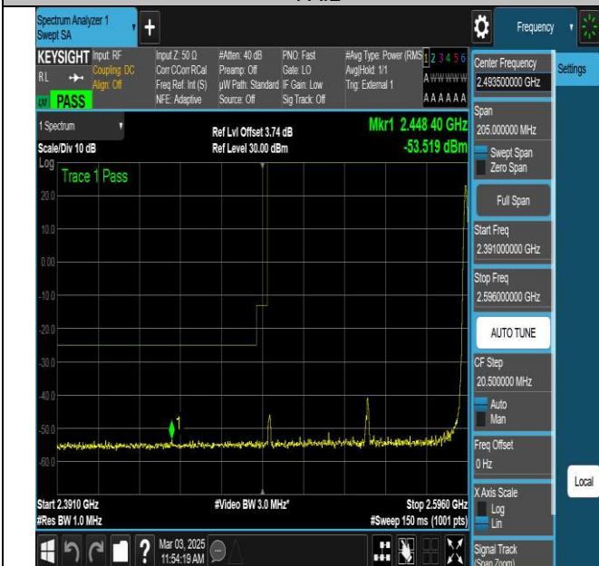
NTNV-N41-PC3-30-100-L-DFT-QPSK-Edge_1RB_Right-Ant1- PASS
