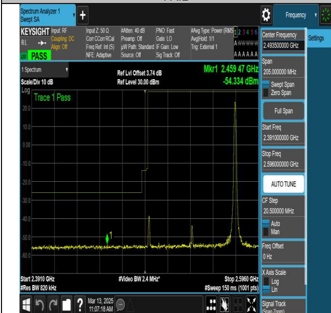
NTNV-N41-PC3-30-80-L-DFT-QPSK-Edge_1RB_Right-Ant1- PASS
