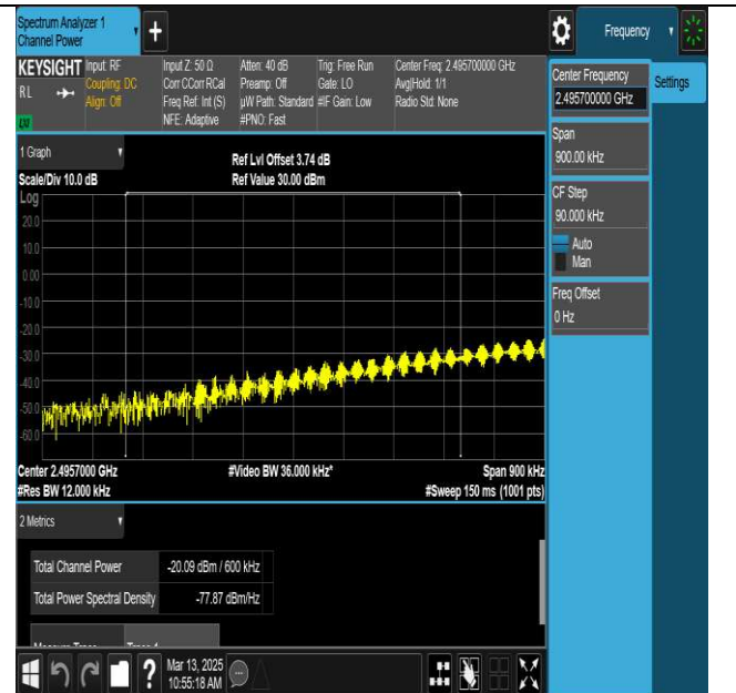
NTNV-N41-PC3-30-60-L-DFT-QPSK-Edge_1RB_Left-Ant1- PASS
