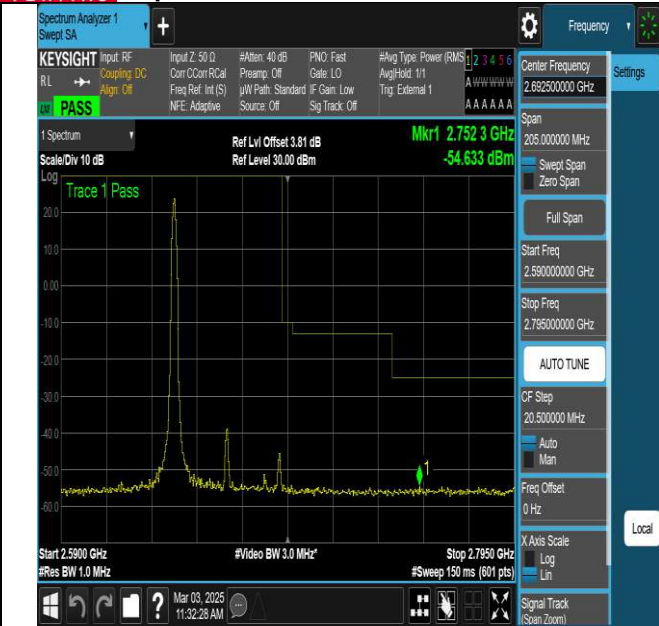
NTNV-N41-PC3-30-50-H-DFT-QPSK-Edge_1RB_Left-Ant1-PASS
