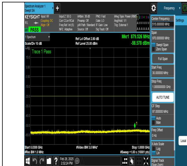
NTNV-N41-PC3-30-10-L-DFT-QPSK-Edge_1RB_Left-Ant1-PASS
