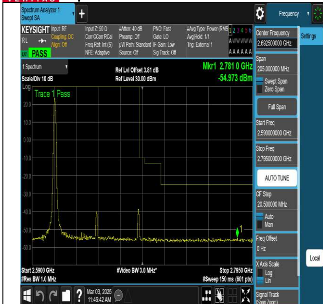
NTNV-N41-PC3-30-80-H-DFT-QPSK-Edge_1RB_Left-Ant1-PASS
