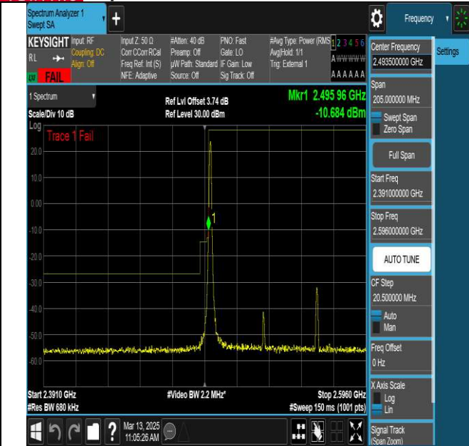
NTNV-N41-PC3-30-70-L-DFT-QPSK-Edge_1RB_Left-Ant1-FAIL
