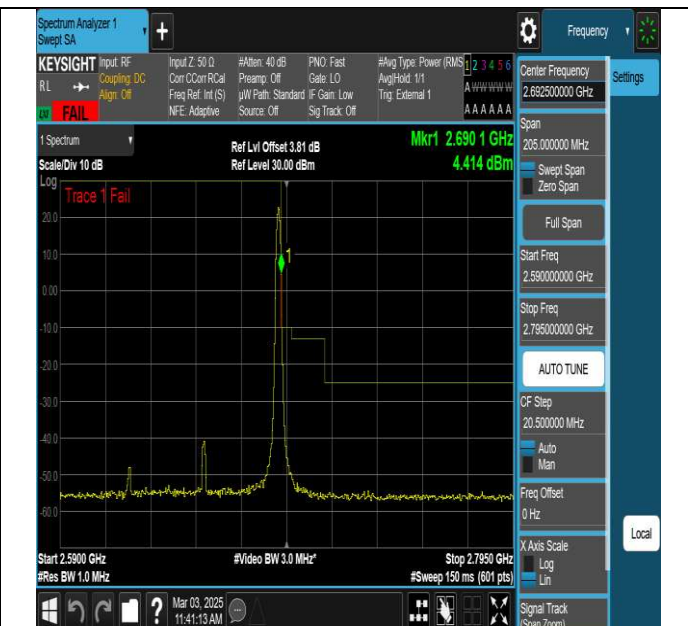
NTNV-N41-PC3-30-70-H-DFT-QPSK-Edge_1RB_Right-Ant1-FAIL
