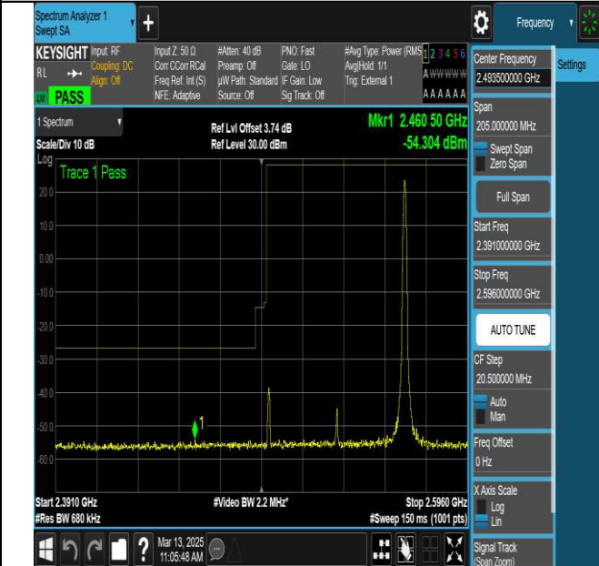
NTNV-N41-PC3-30-70-L-DFT-QPSK-Edge_1RB_Right-Ant1-PASS
