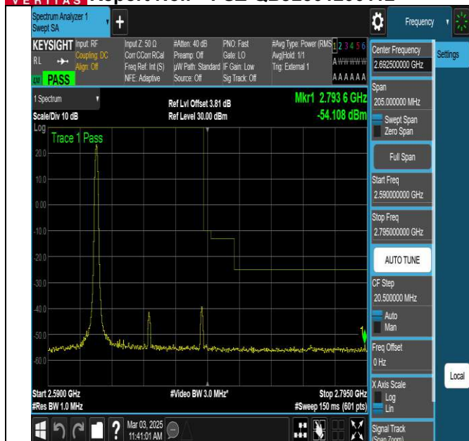
NTNV-N41-PC3-30-70-H-DFT-QPSK-Edge_1RB_Left-Ant1-PASS
