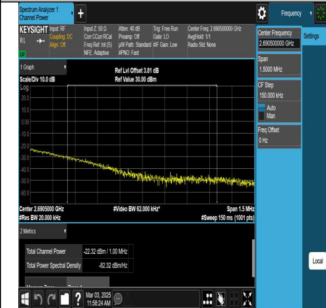
NTNV-N41-PC3-30-100-H-DFT-QPSK-Edge_1RB_Right-Ant1-PASS
