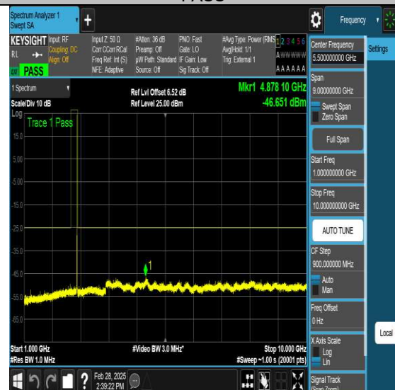
NTNV-N41-PC3-30-10-H-DFT-QPSK-Edge_1RB_Left-Ant1-PASS
