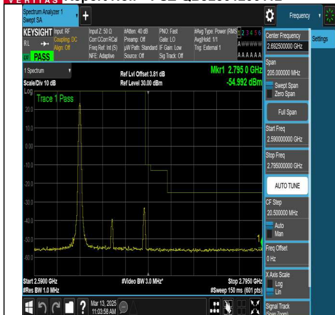
NTNV-N41-PC3-30-60-H-DFT-QPSK-Edge_1RB_Left-Ant1- PASS
