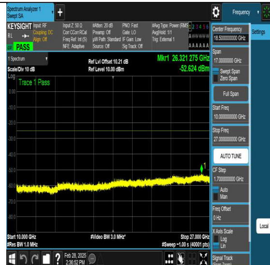
NTNV-N41-PC3-30-10-M-DFT-QPSK-Edge_1RB_Left-Ant1-PASS
