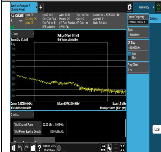
NTNV-N41-PC3-30-80-H-DFT-QPSK-Edge_1RB_Right-Ant1-PASS
