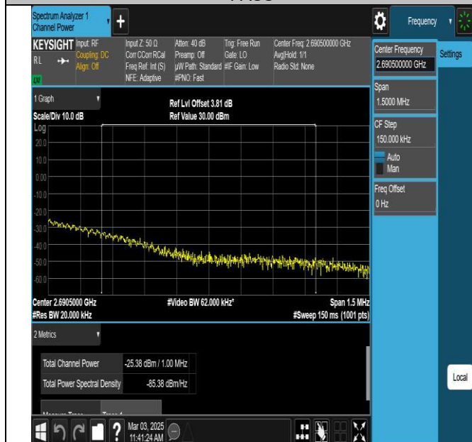
NTNV-N41-PC3-30-70-H-DFT-QPSK-Edge_1RB_Right-Ant1-PASS
