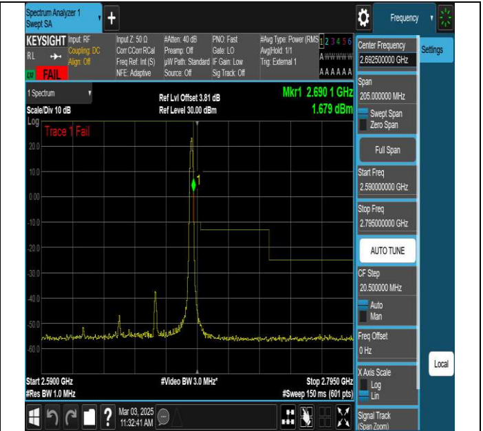
NTNV-N41-PC3-30-50-H-DFT-QPSK-Edge_1RB_Right-Ant1-FAIL
