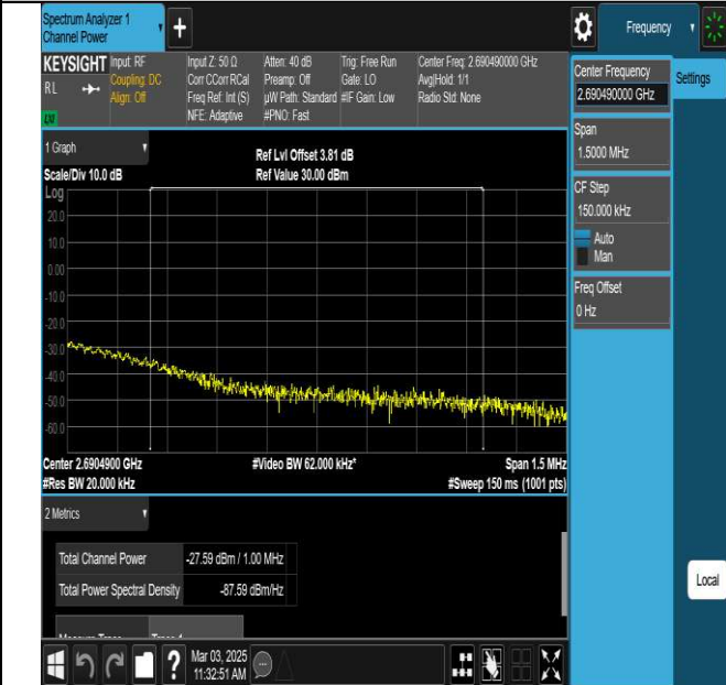
NTNV-N41-PC3-30-50-H-DFT-QPSK-Edge_1RB_Right-Ant1-PASS
