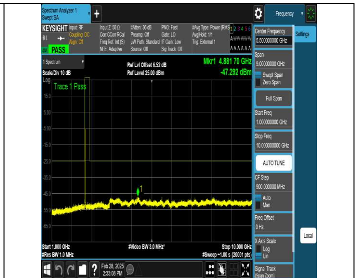
NTNV-N41-PC3-30-10-L-DFT-QPSK-Edge_1RB_Left-Ant1-PASS
