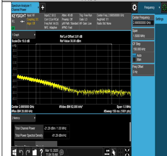
NTNV-N41-PC3-30-60-H-DFT-QPSK-Edge_1RB_Right-Ant1- PASS
