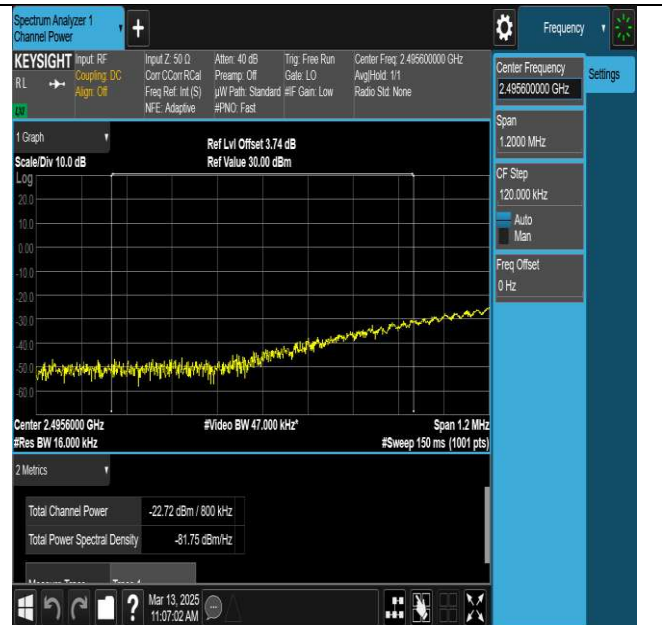
NTNV-N41-PC3-30-80-L-DFT-QPSK-Edge_1RB_Left-Ant1- PASS
