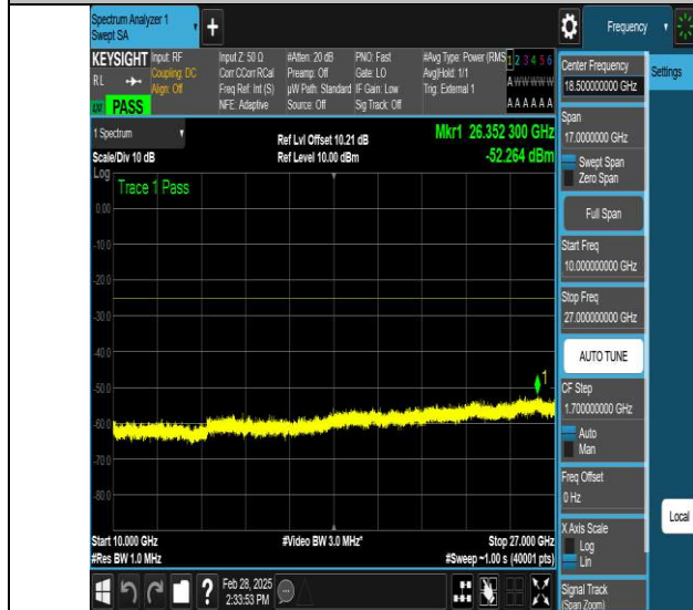
NTNV-N41-PC3-30-10-L-DFT-QPSK-Edge_1RB_Left-Ant1-PASS
