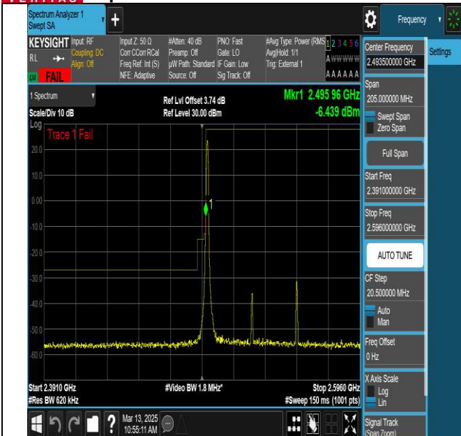
NTNV-N41-PC3-30-60-L-DFT-QPSK-Edge_1RB_Left-Ant1- FAIL
