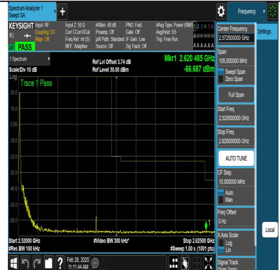
NTNV-N7-PC3-15-50-H-DFT-QPSK-Edge_1RB_Left-Ant1-
