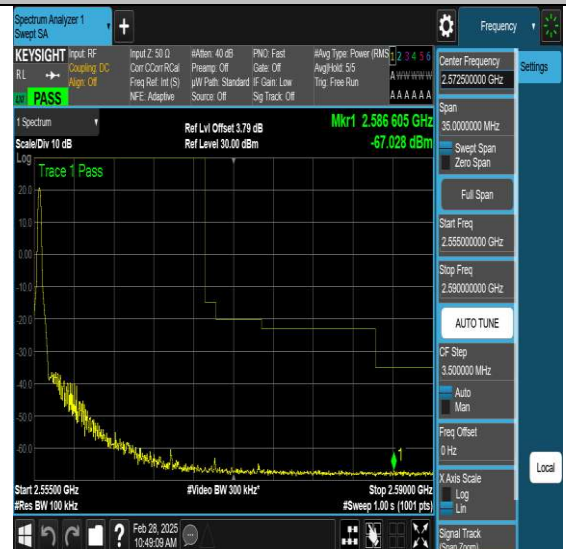
NTNV-N7-PC3-15-15-L-DFT-QPSK-Edge_1RB_Right-Ant1-PASS
