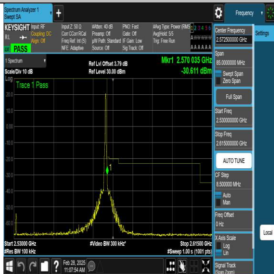
NTNV-N7-PC3-15-40-H-DFT-QPSK-Edge_1RB_Right-Ant1-PASS
