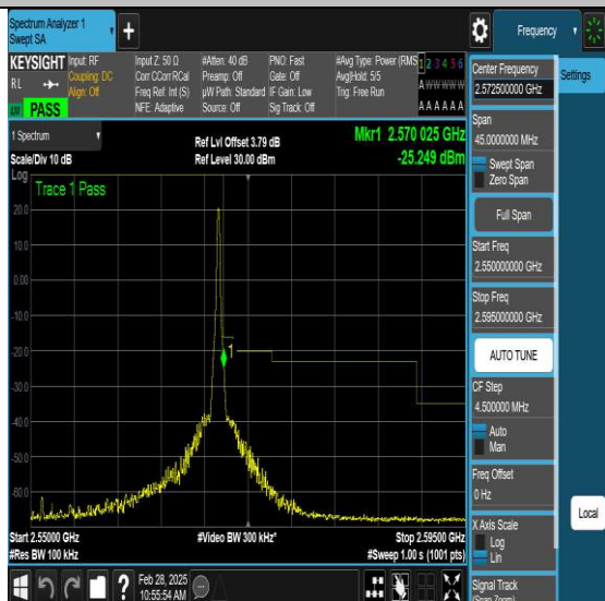
NTN-N7-PC3-15-20-H-DFT-QPSK-Edge_1RB_Right-Ant1-PASS
