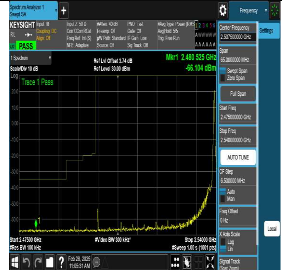
NTNV-N7-PC3-15-40-L-DFT-QPSK-Edge_1RB_Right-Ant1-PASS
