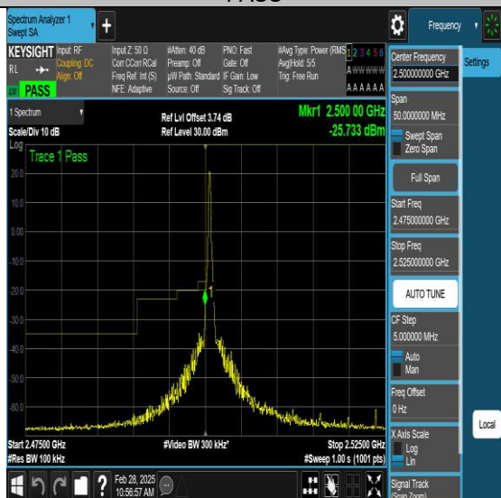
NTN-N7-PC3-15-25-L-DFT-QPSK-Edge_1RB_Left-Ant1-
