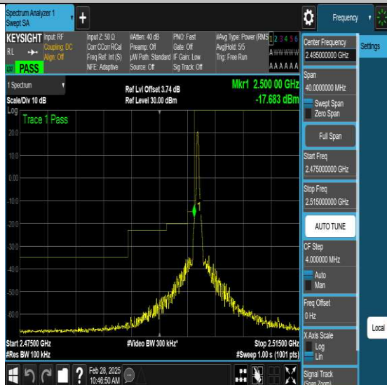
NTNV-N7-PC3-15-15-L-DFT-QPSK-Edge_1RB_Left-Ant1-PASS
