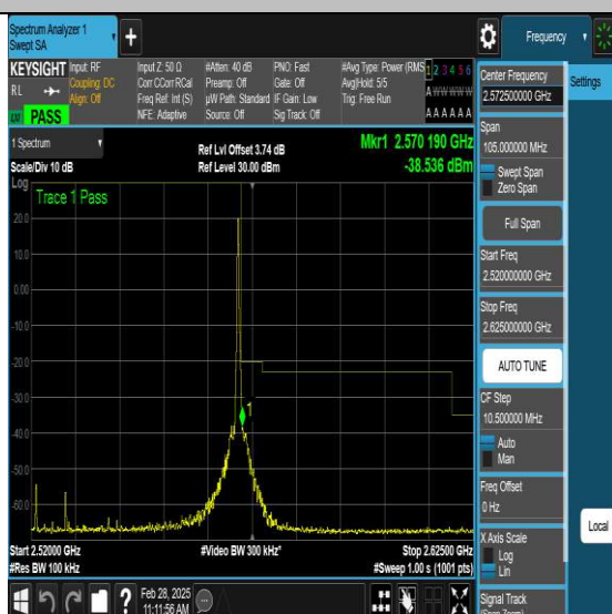
NTNV-N7-PC3-15-50-L-DFT-QPSK-Outer_Full-Ant1-PASS
