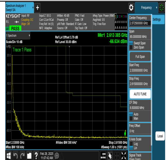
NTNV-N7-PC3-15-40-H-DFT-QPSK-Edge_1RB_Left-Ant1-PASS
