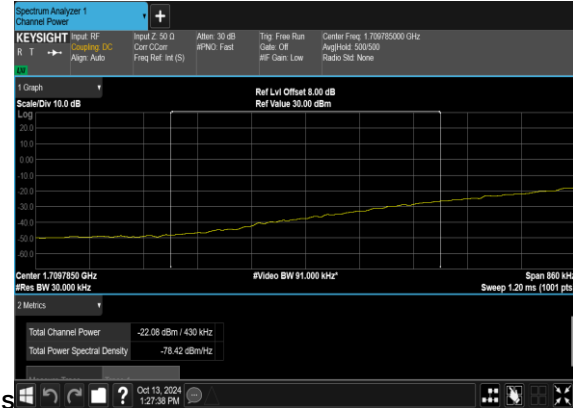
N66(40M)_DFT-s- OFDM_QPSK_Edge_1RB_Left_Low_CH_CHP_PAS
