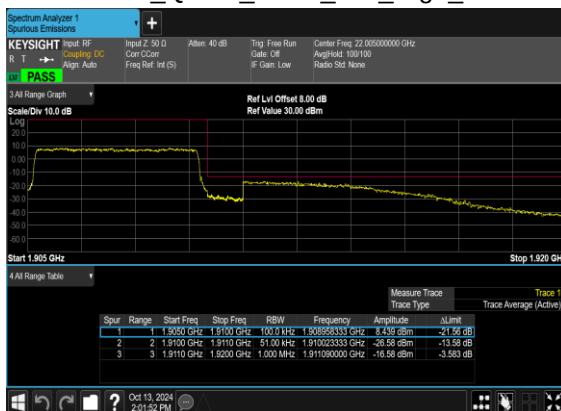
N2(5M)_DFT-s- OFDM_QPSK_Outer_Full_High_CH
