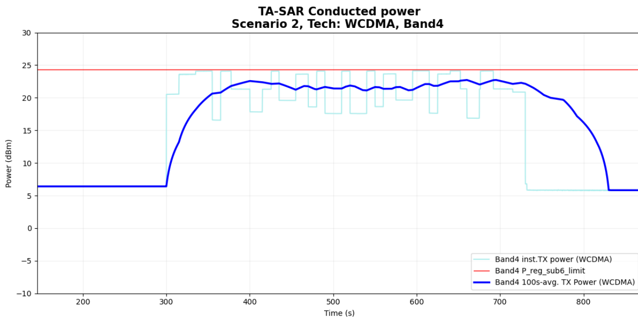
Figure 6- 17 Time-averaged conducted TX power over time
