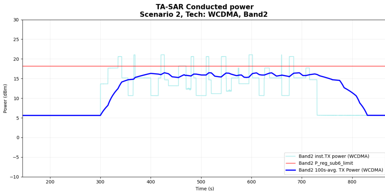
Figure 6- 21 Time-averaged conducted TX power over time
