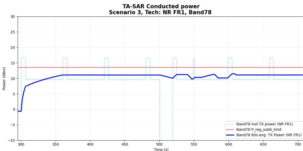
Figure 6- 39 Time-averaged conducted TX power over time
