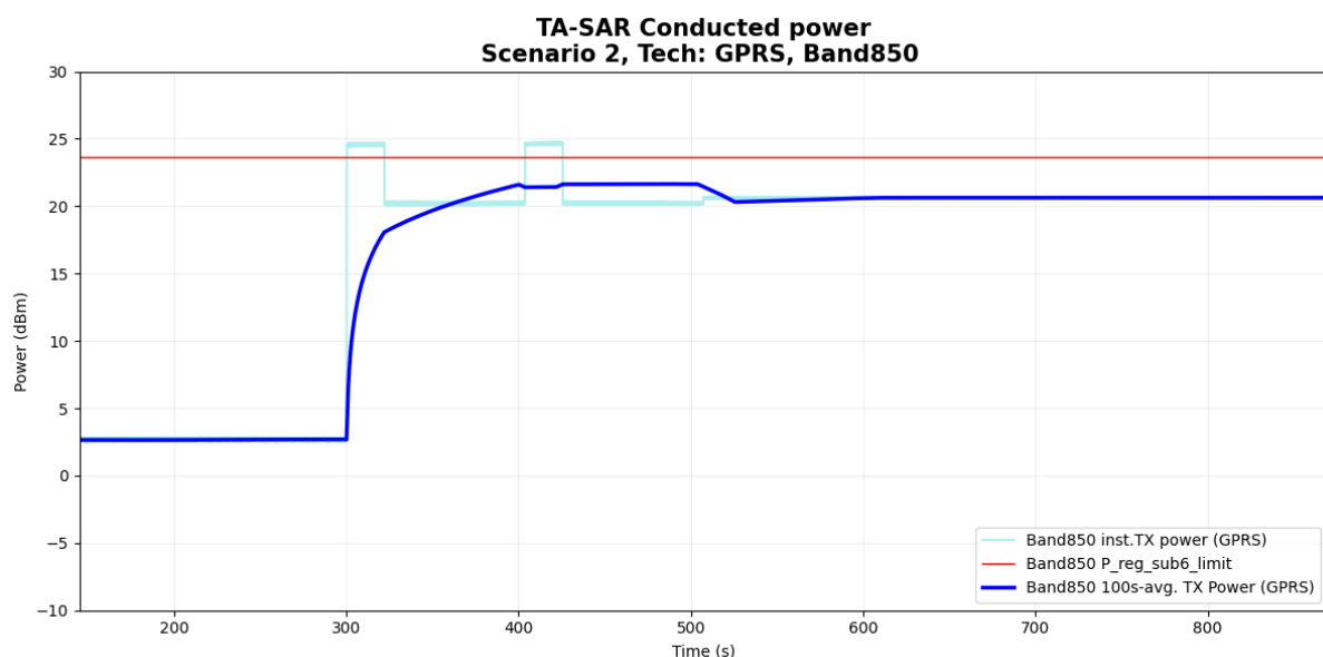
Figure 6- 7 Time-averaged conducted TX power over time
