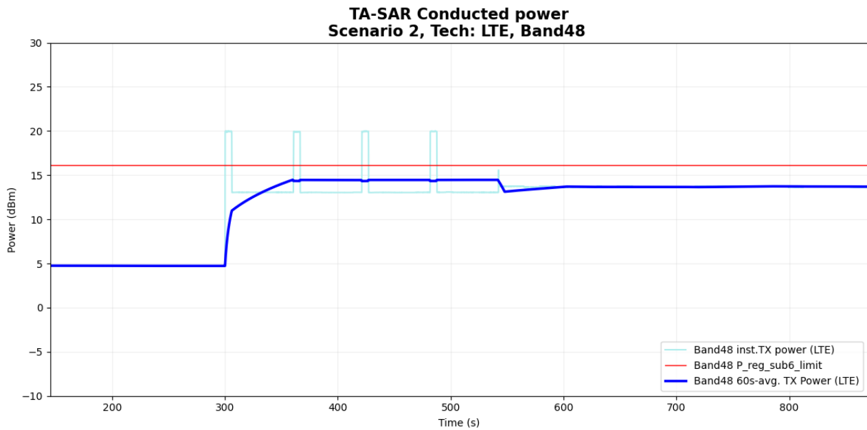
Figure 6- 27 Time-averaged conducted TX power over time
