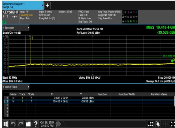
N38(25M)_DFT-s-OFDM_QPSK_Edge_1RB_Left_Mid_CH
