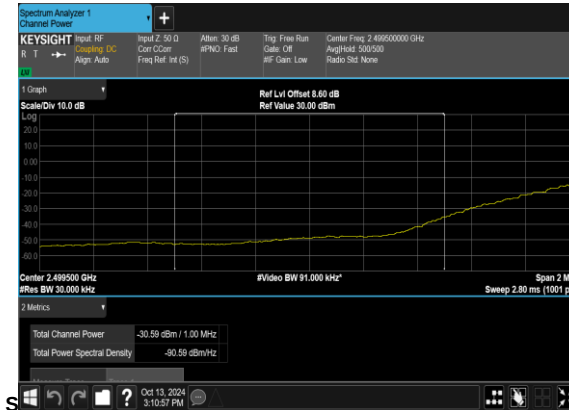
N7(50M)_DFT-s- OFDM_BPSK_Edge_1RB_Left_Low_CH_CHP_PAS
