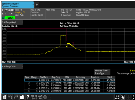
N7(5M)_DFT-s- OFDM_QPSK_Outer_Full_High_CH
