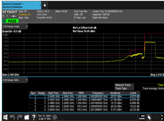
N7(5M)_DFT-s- OFDM_BPSK_Outer_Full_Low_CH
