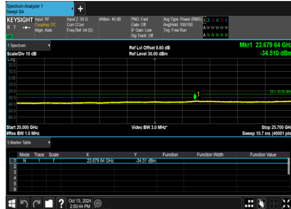
N7(50M)_DFT-s- OFDM_QPSK_Edge_1RB_Left_Low_CH
