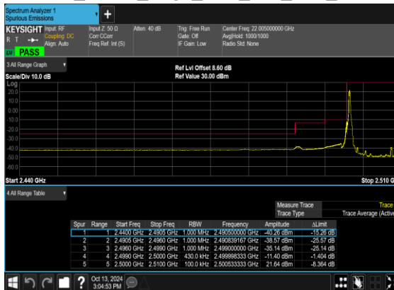
N7(20M)_DFT-s- OFDM_QPSK_Edge_1RB_Left_Low_CH
