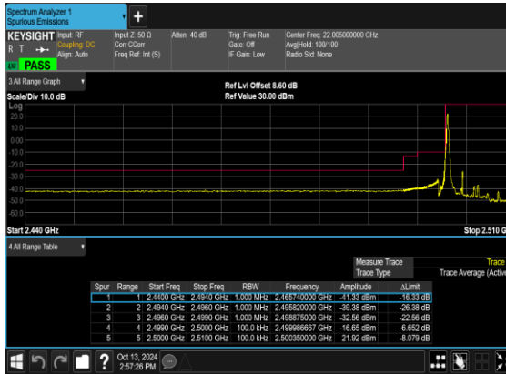
N7(5M)_DFT-s- OFDM_BPSK_Edge_1RB_Left_Low_CH
