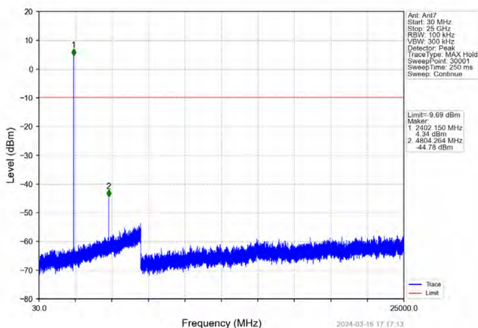
8DPSK_3DH5_LCH_2402MHz_Ant7_NTNV
