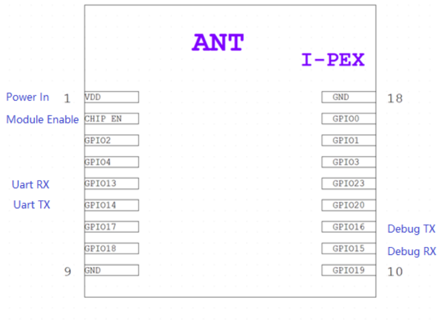
figure 2-1. MHCWB4P-B pin distribution
