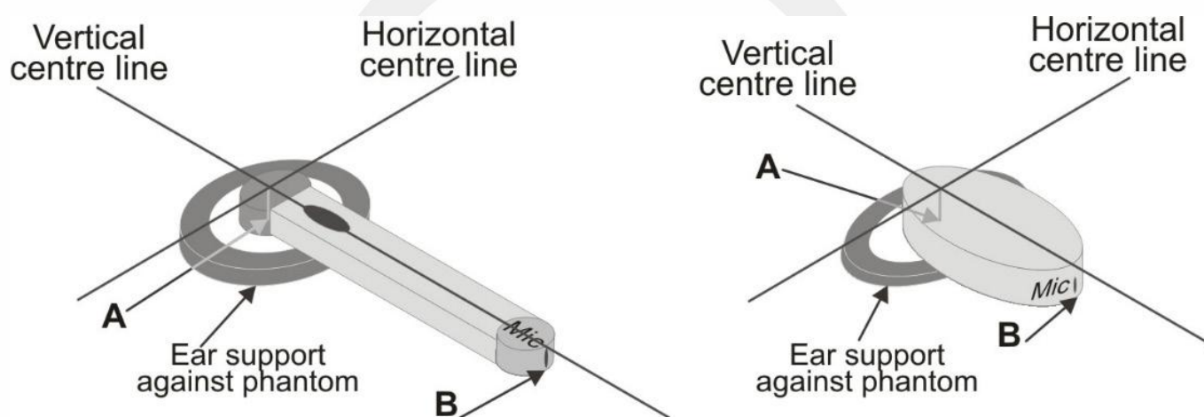
Fig-4.1 An alternative form factor DUT and standard coordinate and reference points applied
