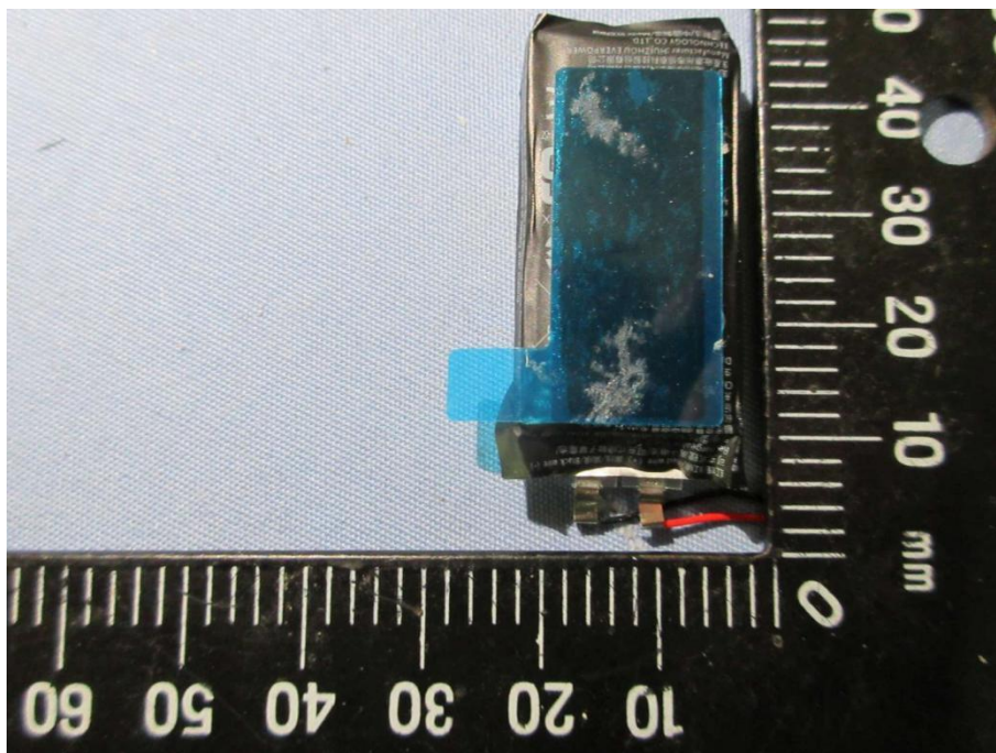
BATTERY 2 (TOP) - Model: HT782039
