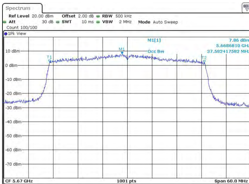
11AX40MIMO-484T Ant2 5670
