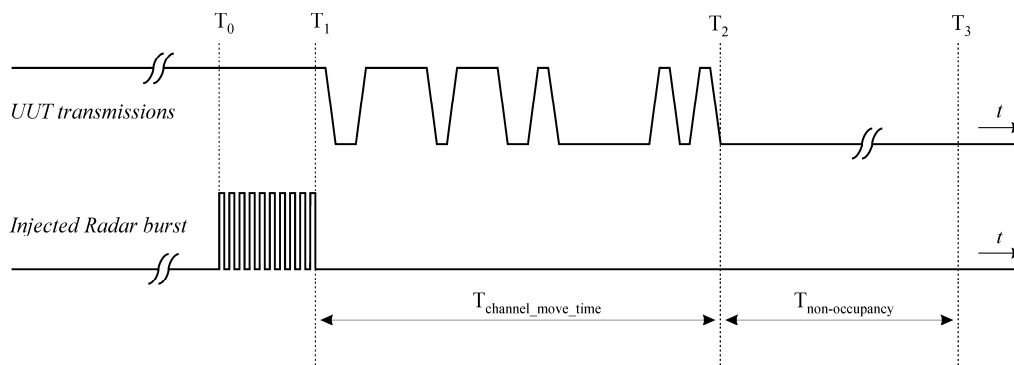
Figure 2: Example of Channel Closing Transmission Time & Channel Closing Time
