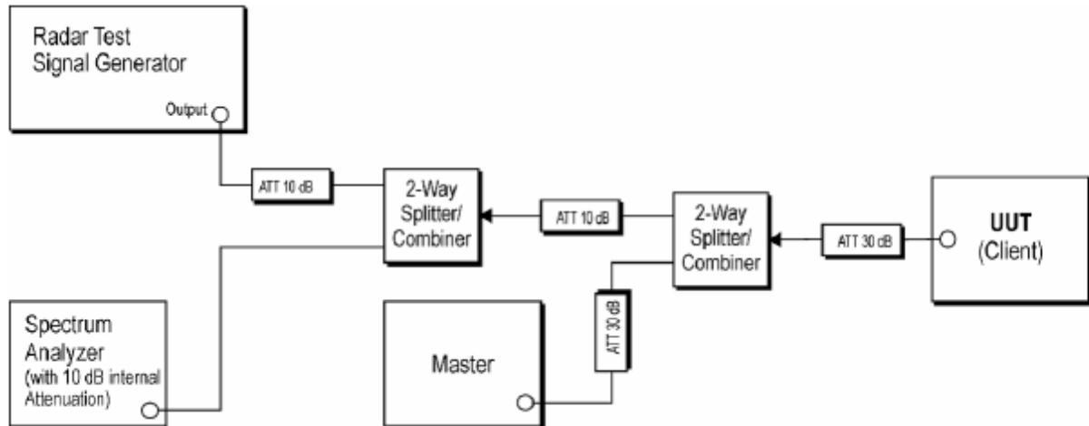
Figure 1: Example Conducted Setup where UUT is a Client and Radar Test Waveforms are injected into the Client
