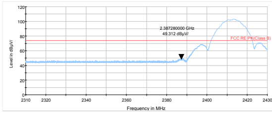
802.11b-Channel 1 Peak
