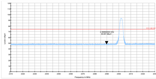
BLE Channel 0 Peak
