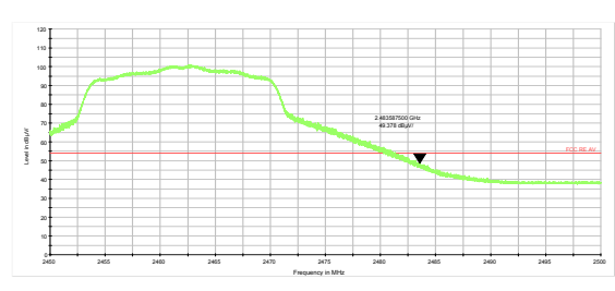
802.11g-Channel 11 Average
