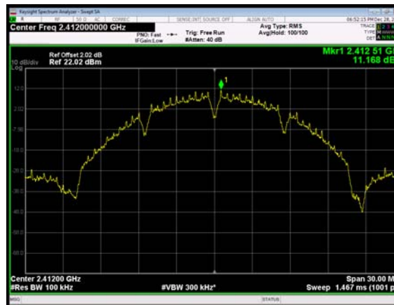
802.11b, Channel No.: 1
