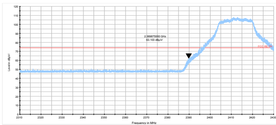
802.11g-Channel 1 Peak
