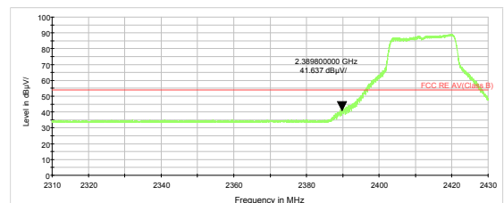
802.11n HT20 -Channel 1 Average
