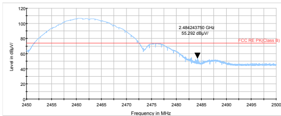
802.11b-Channel 11 Peak
