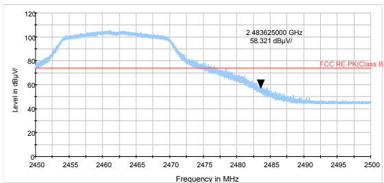
802.11g-Channel 11 Peak
