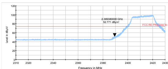
802.11n HT20 -Channel 1 Peak
