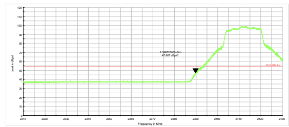
802.11g-Channel 1 Average
