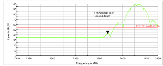
802.11b-Channel 1 Average
