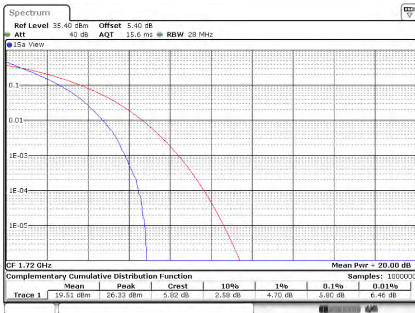
Band66-20MHz-QPSK-132072-100RB#0
