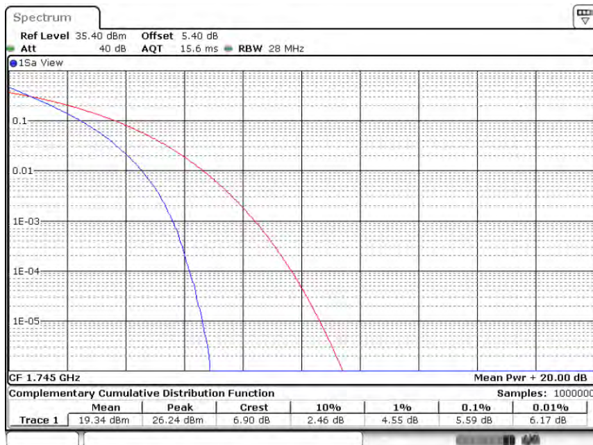
Band66-20MHz-QPSK-132322-100RB#0
