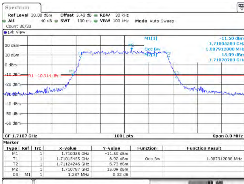
Band66-1.4MHz-QPSK-131979-6RB#0-1.088
