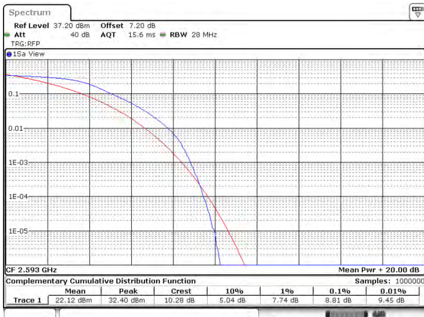
Band41-20MHz-QPSK-40620-100RB#0
