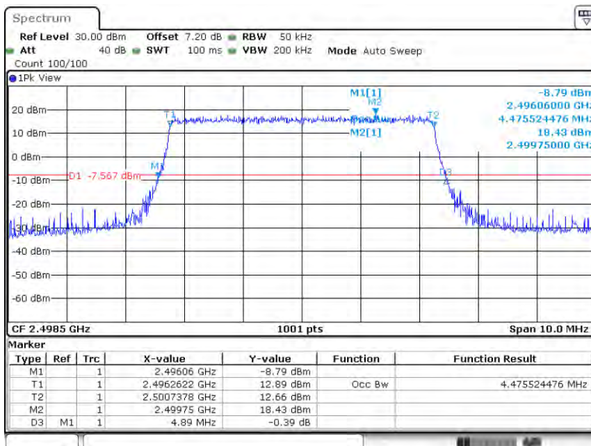
Band41-5MHz-QPSK-39675-25RB#0-4.476
