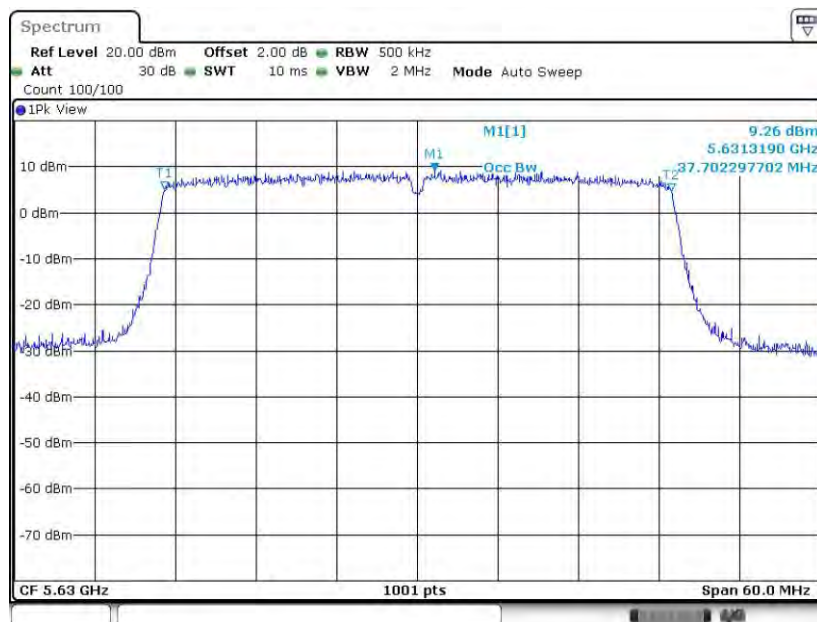
11AX40MIMO-484T Ant2 5630
