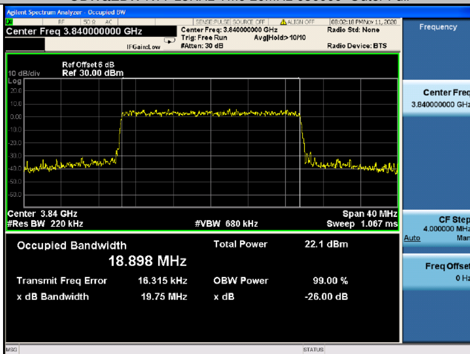
OBW&amp;EBW N77 15KHz TM1 40MHz 656000 Outer Full
