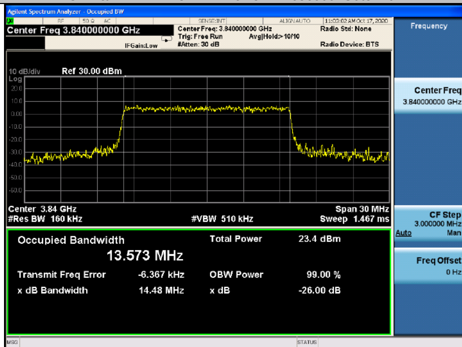
OBW&amp;EBW N77 15KHz TM6 15MHz 656000 Outer Full
