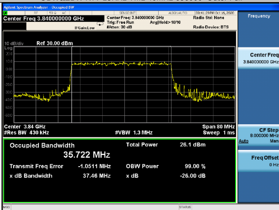
OBW&amp;EBW N77 15KHz TM2 40MHz 656000 Outer Full
