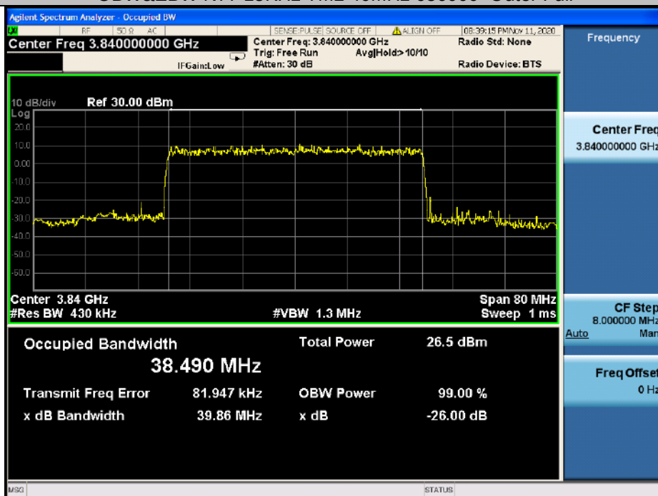
OBW&amp;EBW N77 15KHz TM3 40MHz 656000 Outer Full
