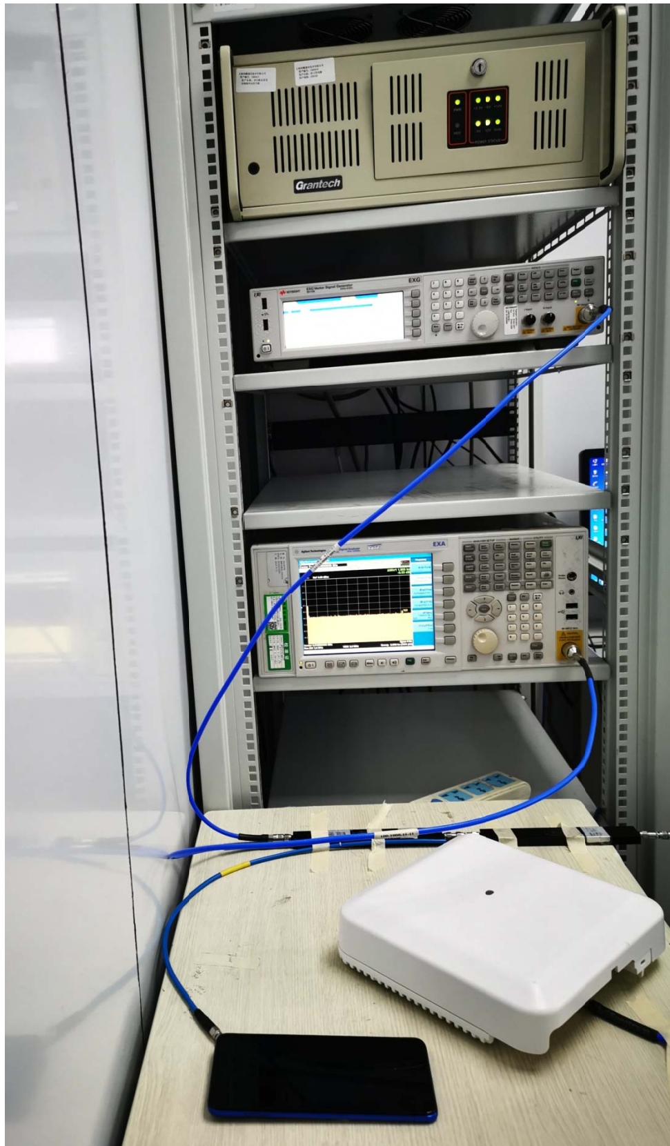
Picture 1 Test Setup
