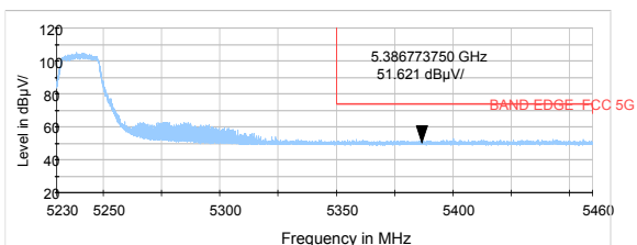
802.11a-Channel 48: Average
