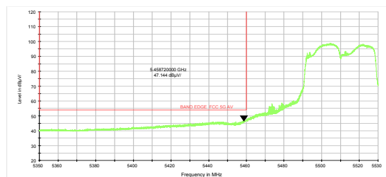
802.11n HT40-Channel 102: Average
