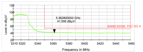
802.11a-Channel 64: Average
