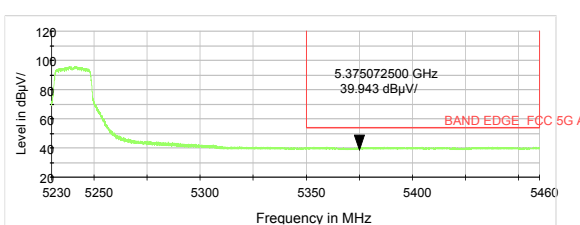
802.11n HT20-Channel 48: Peak
