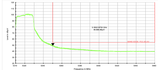
802.11n HT20-Channel 64: Average
