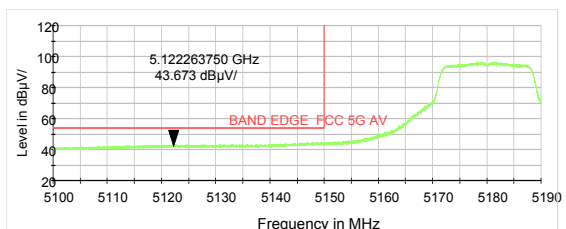
802.11a-Channel 36: Average
