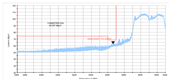
802.11n HT40-Channel 102: Peak
