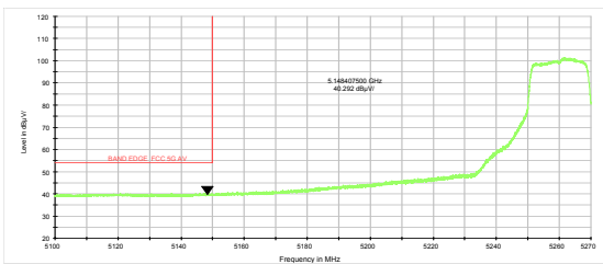
802.11n HT20-Channel 52: Average
