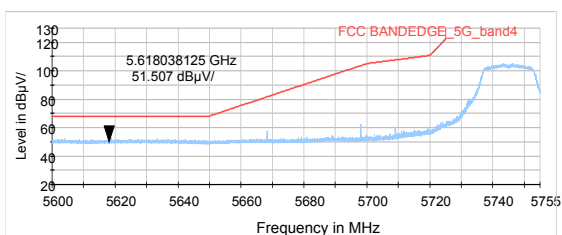
802.11n HT20-Channel 149: Peak
