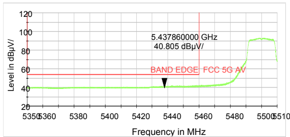
802.11a-Channel 100: Average
