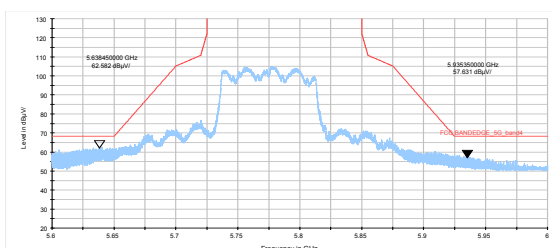
802.11ac VHT80- Channel 155: Peak
