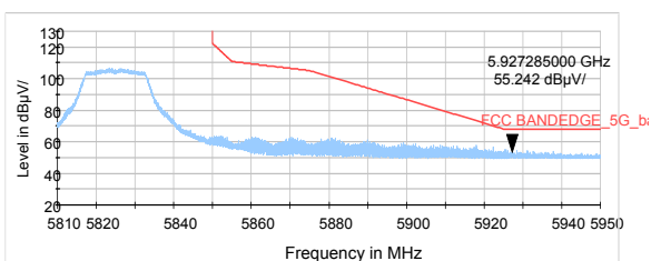
802.11n HT20-Channel 165: Peak
