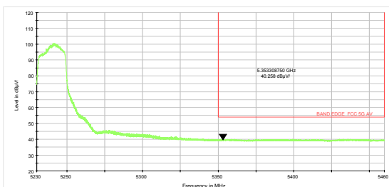
802.11n HT20-Channel 48: Average
