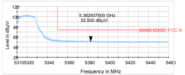
802.11a-Channel 64: Average
