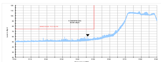
802.11n HT20-Channel 36: Peak
