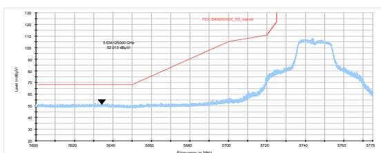
802.11n HT20-Channel 149: Peak
