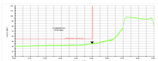
802.11n HT20-Channel 36: Average
